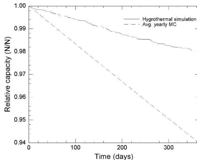
Figure 6.—Relative capacity as a function of time (same parameters as Fig. 2) for two cases, based on the yearly average moisture content, or based on the instantaneous moisture content from a hygrothermal simulation.
