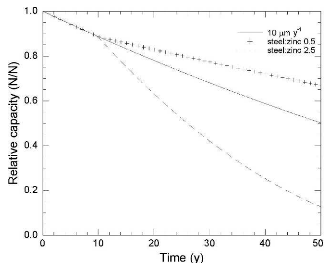
Figure 3.—Relative capacity as a function of time for an 8d common galvanized fastener corroding at 10 \mu\text{m y}^{-1} and exhibiting a Mode IV failure. Different lines represent different relative steel:galvanized steel corrosion rate ratios.
