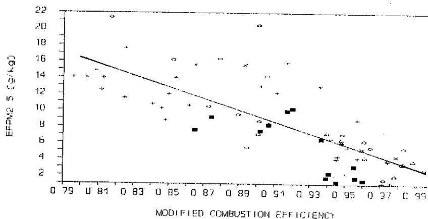
Fig. 8. Particulate matter emission factors for particles of less than 2.5 micrometers diameter (PM2.5) as a function of modified combustion efficiency for all fires.
