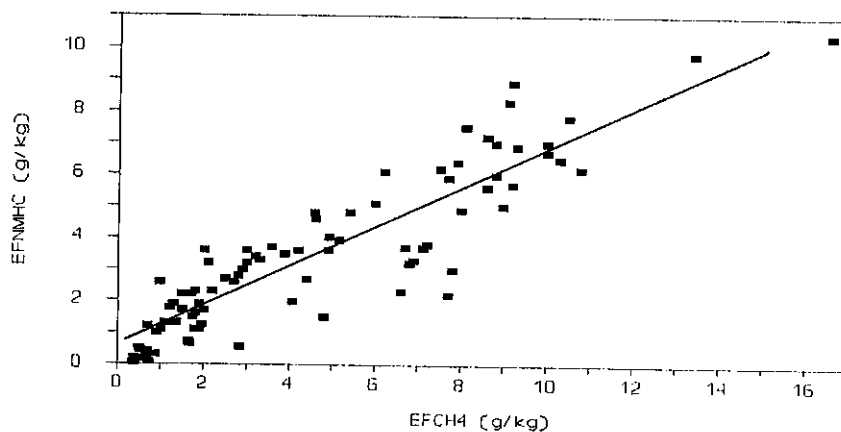
Fig. 7. Emission factors for nonmethane hydrocarbons (NMHC) as a function of emission factors for \text{CH}_4 for all fires.
