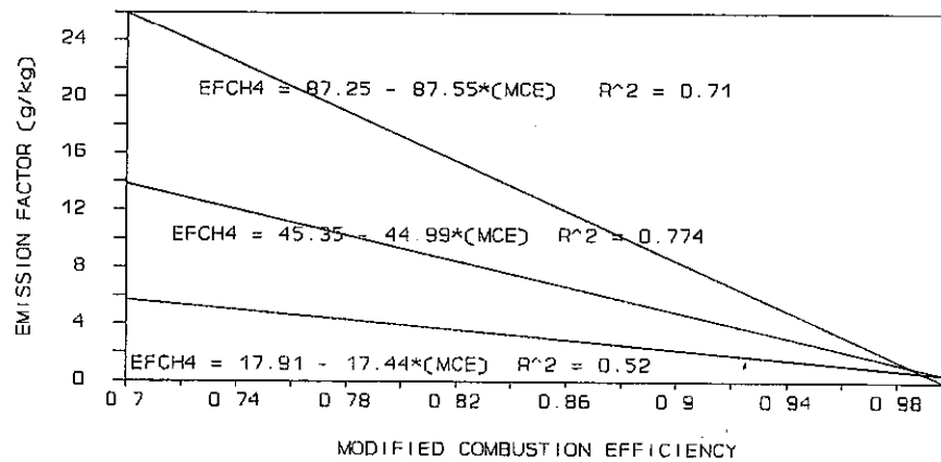
Fig. 6. Models for estimating emission factors for CH 4 by fuel type as a function of modified combustion efficiency.
