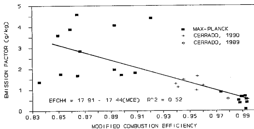
Fig. 3. CH 4 emissions for fires in grass, cerrado, savannah, and agricultural fuel types.
