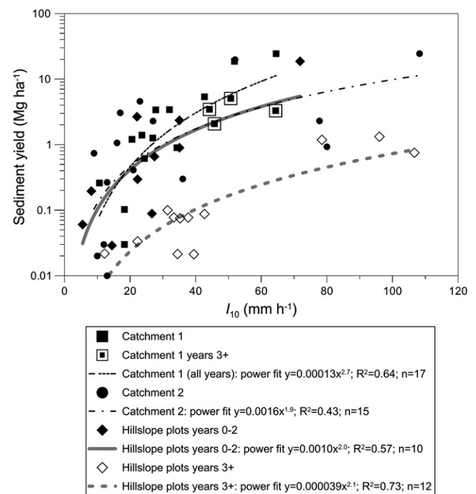
Fig. 6. Event sediment yields versus 10-min maximum intensity ( I_{10} ) for the Hayman fire control sites. Catchment 1 is from the current study. Catchment 2 is another control catchment in the Hayman fire located closer to the hillslope plots; the same methods were used as in the current study (Wagenbrenner et al., in preparation). The catchment fit lines are based on all data at each catchment; the open symbols indicate the data collected after post-fire year 2 for comparison to the hillslope plot data for the same period. The plot data are the mean sediment yields from the control hillslope plots in part I of the current study (Robichaud et al., 2013). The plot data are shown in two groups: post-fire years 0–2 and post-fire years 3–7; the fit lines were modeled separately for each group.
