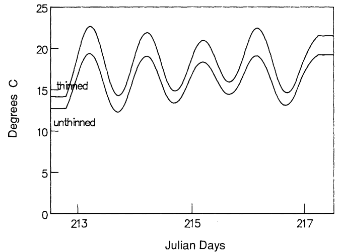
Figure 4 —Smoothed curves for a 5-day period contrasting bark surface temperatures on the south side of two lodgepole pine trees between a thinned and unthinned stand.
