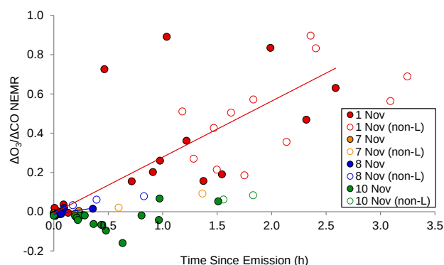
Fig. 12. \Delta\text{O}_3/\Delta\text{CO} NEMR vs. time since emission (h). Airborne measurements were collected up to \sim 2.5 h downwind. All the SC fires that we were able to collect downwind data on are shown: Block 9b (1 November, red), Georgetown (7 November, orange), Francis Marion (8 November, blue), and Bamberg (10 November, green). The y-intercept of the trendlines for 1 and 8 November is forced to the average \Delta\text{O}_3/\Delta\text{CO} NEMR at time t = 0 h for each fire. All trendlines represent only pseudo-Lagrangian data points. The 7 November data did not have enough points to constrain a line and the 10 November data was clearly non-linear. Solid circles reflect data that were Lagrangian while open circles labeled “non-L” represent non-Lagrangian samples collected on that respective day.
