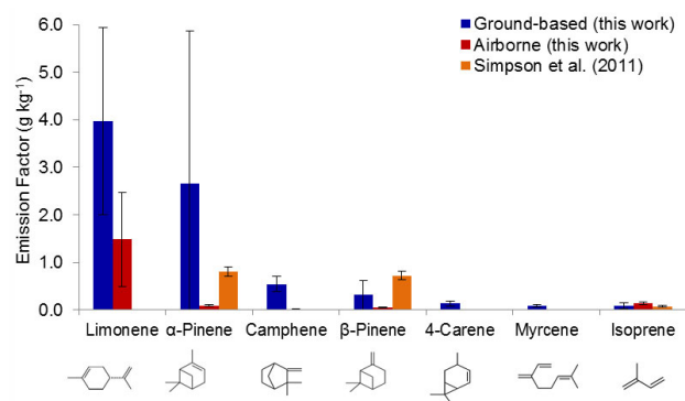
Fig. 7. Emission factors (g kg -1 ) of monoterpenes and isoprene measured in this work from ground-based (blue) and airborne (red) platforms. Molecular structures are shown below each compound. We compare with data from Simpson et al. (2011) who measured \alpha -pinene, \beta -pinene and isoprene only from an airborne platform (orange). Error bars represent the 1- \sigma standard deviation in EF.
