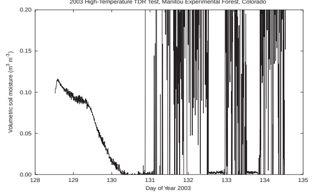
Figure 4: Seven days of soil moisture probe data at the campfire site. The fire was initiated about 1 pm (MDT) May 8 (day 128), 2003. The probe began to fail about day 131, but performed intermittently on days 132 and 133. The probe was retrieved on day 134.
