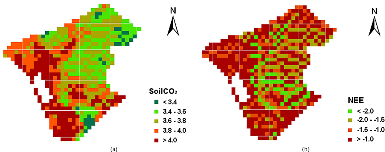
Figure 4. (a) Spatial differences in annual average soil \text{CO}_2 flux ( \text{Mg}\cdot\text{C}\cdot\text{ha}^{-1}\cdot\text{yr}^{-1} ) in the period from 1950-2007; (b) Spatial differences in annual average NEE ( \text{Mg}\cdot\text{C}\cdot\text{ha}^{-1}\cdot\text{yr}^{-1} ) in the period from 1950-2007.
