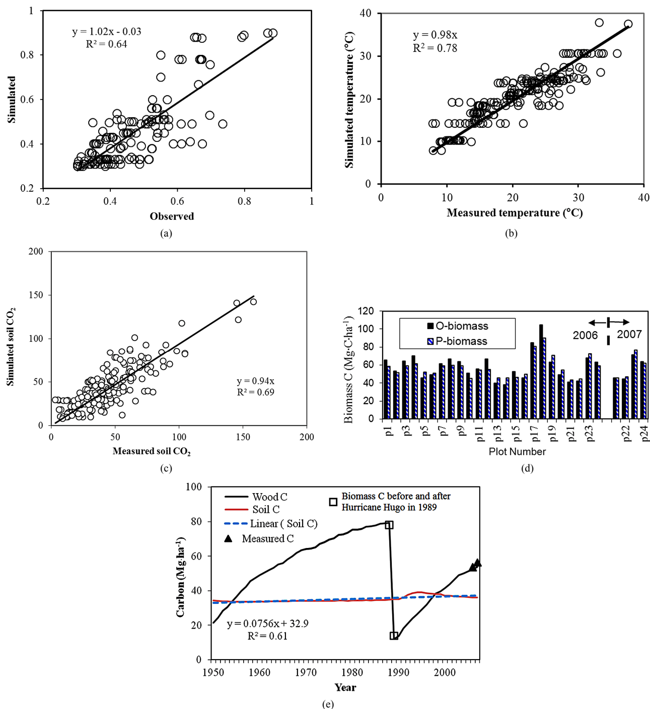
Figure 3. (a) Observed and simulated daily soil moisture (0 - 1) for eight plots (plot average) ( n = 216 ); (b) Observed and simulated daily soil temperature (°C) for eight plots (plot average) ( n = 216 ); (c) Observed and simulated soil CO 2 fluxes (kg·C·ha -1 ·d -1 ) for eight plots (plot average) ( n = 200 ); (d) Observed and simulated aboveground biomass (Mg·C·ha -1 ) for plots p1 - p24 in 2006 and p21 - p24 in 2007 (O-biomass is the measured biomass C; P-biomass is the simulated); (e) Temporal changes in biomass and mineral soil organic carbon (Mg·C·ha -1 ) within a depth of 30 cm; ([Wood C] is simulated annual mean aboveground biomass C for the 58-year period from 1950-2007; [Measured C] is the estimated aboveground biomass for 2006 and 2007 using plot average based on the biomass measurements in 2006 and 2007, respectively; [Biomass C before and after Hurricane Hugo in 1989] is the aboveground biomass C estimated by Hook et al. (1996); n = 39 for the linear (Soil C) regression).
