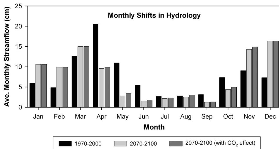
Figure 2. Comparison between measured monthly discharge for 1970–2000 and simulated mean monthly discharge for 2070–2100 with and without considering \text{CO}_2 effects on vegetation. Note the future climate-change scenario depicted in these results is from HadCM3 A1fi.
