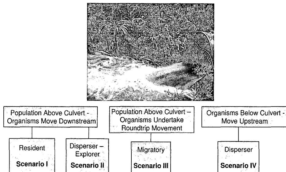
Figure 1. General model of potential effects of the presence of culverts on aquatic organism populations. Culvert photograph by David Leer, Oregon State University.
