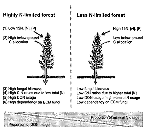
Figure 6. Summary of the relationship between black spruce \delta^{15}\text{N} values, soil N status, and the abundance and activity of ectomycorrhizal (ECM) fungi. Highly N-limited forests: (1) exhibit low (for example, very negative) needle \delta^{15}\text{N} values as well as N and P concentrations (Figure 1); (2) high belowground C allocation is presumed to be larger in these stands based on several studies in other boreal forests (Högberg and others 2003, 2010, 2011; Nilsson and Wallander 2003); (3) high relative fungal biomass follows the literature supported predictions (2) and is positively correlated with (4); (4) high C:N ratios were positively correlated with fungal biomass due to lower total (Figure 4) and dissolved N in organic soils; (5) high dissolved organic N (DON) is positively correlated with foliar N concentrations (Table 1) but negatively correlated with sporocarp \delta^{15}\text{N} values (Figure 3) and corresponds to the mixing model estimations (Supplementary Table S2); and, (6) usage of DON requires a greater dependency on ECM fungi (Supplementary Table S2).
