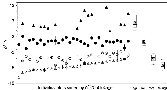
Figure 2. Average ( \pm\text{SE} ) black spruce full sun needle (open triangle), fine root (open circle), bulk organic soil (filled circle), and ECM sporocarp (filled triangle) \delta^{15}\text{N} values across 31 plots in central Alaska. Box plots illustrate overall means (times), medians (line), and 95th percentiles. Points are arbitrarily arrayed according to average foliar \delta^{15}\text{N} values to illustrate the lack of strong covariance among components. Only foliar \delta^{15}\text{N} was significantly correlated with root \delta^{15}\text{N} ( \delta^{15}\text{N}_{\text{foliar}} = -4.69 + 0.51\delta \times \delta^{15}\text{N}_{\text{root}} , R^2 = 0.30 , P = 0.01 ). The slope for foliar \delta^{15}\text{N} (0.16) is nearly twice that of both the ECM sporocarps and black spruce fine roots (0.09), although not statistically different. Across all plots, ecosystem components were different from one another (paired t test, P < 0.001 ) and the mean isotopic differences between foliage and root, foliage and soil, and foliage and fungal \delta^{15}\text{N} values were -2.4 , -7.7 , and -13.8\text{‰} , respectively.
