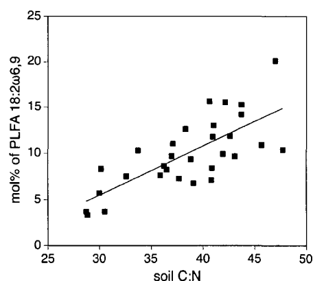
Figure 4. Relation among C:N ratios of the organic black spruce soils with the mol% phospholipid fatty acid (PLFA) 18:2 \omega 6,9, a metric of relative fungal abundance ( R^2 = 0.54 , P < 0.0001 ).
