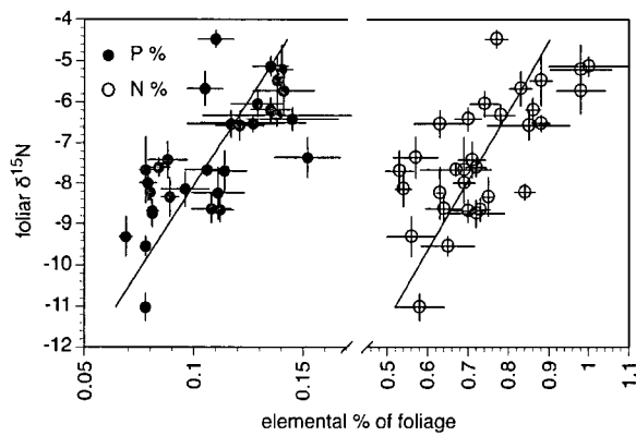
Figure 1. Relationships between \delta^{15}\text{N} (‰) and N and P content (%) of full sun needles ( n = 3 ) collected from black spruce ( Picea mariana ) trees in 31 plots in central Alaska. Phosphorus % ( \mu\text{g g}^{-1} ): R^2 = 0.53 , P < 0.001 ; Nitrogen %: R^2 = 0.46 , P < 0.001 .
