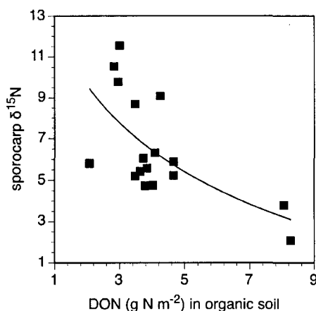
Figure 3. Relation among organic soil DON content and fungal sporocarp \delta^{15}\text{N} values from 17 plots in central Alaska. R^2 = 0.38 , f(\chi) = -4.62 \times \ln(\chi) + 12.8 , P = 0.009 .
