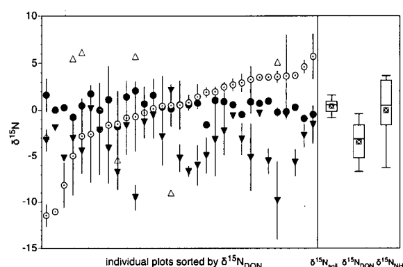
Figure 5. Mean ( n = 3 , \pm\text{SE} ) soil N \delta^{15}\text{N} values from dissolved organic N (DON, open circles), ammonium ( \text{NH}_4^+ , filled triangles), and bulk organic soils (filled circles), and nitrate ( \text{NO}_3^- , open triangles) across 31 plots in central Alaska. The \delta^{15}\text{N} values are arbitrarily sorted by \delta^{15}\text{N}_{\text{DON}} values to examine covariance among pools. The figure on the right is the mean (times) and median (line) \pm\text{SE} of the isotope values used in our analysis.
