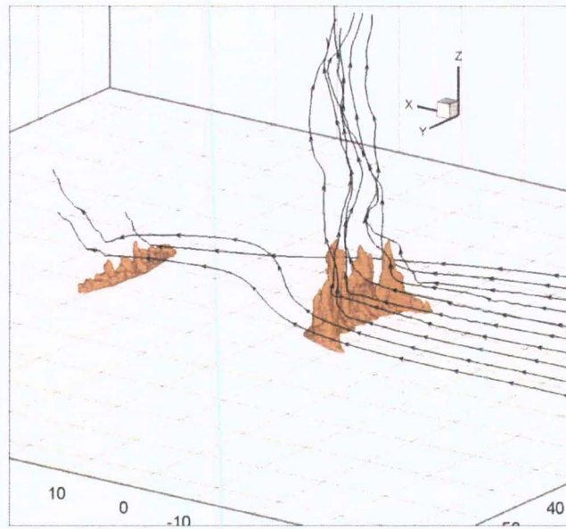
Fig. 4. Streamlines rake emitted at z = 5\text{ m} above the ground level during the propagation of two line fires in grassland (10 m open wind speed: U_{10} = 1\text{ m/s} ).
