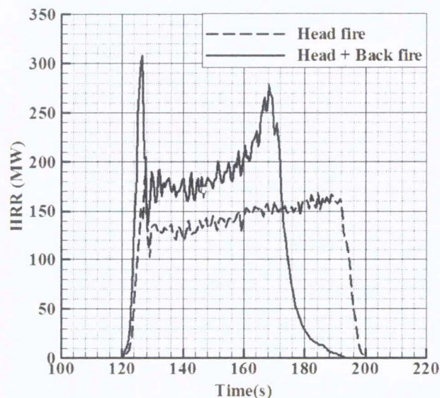
Fig. 5. Heat release rate calculated during after the ignition of one (dashed line) and two (continuous line) in grassland (10 m open wind speed: U_{10} = 1 m/s).
