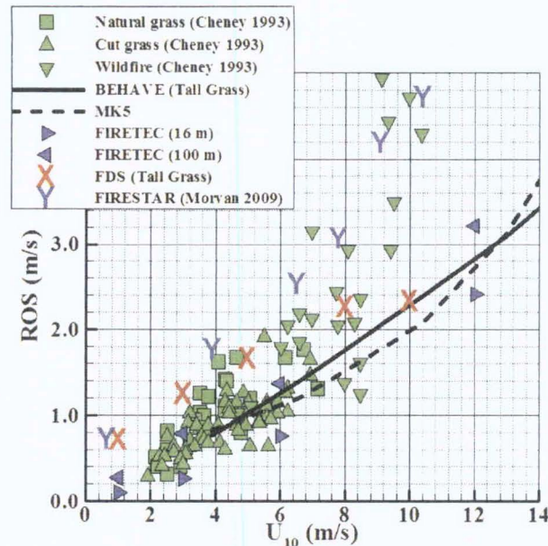
Fig. 1. Rate of spread (ROS) versus 10 m open wind speed ( U_{10} ) for a standalone surface fire propagating through a grassland.
