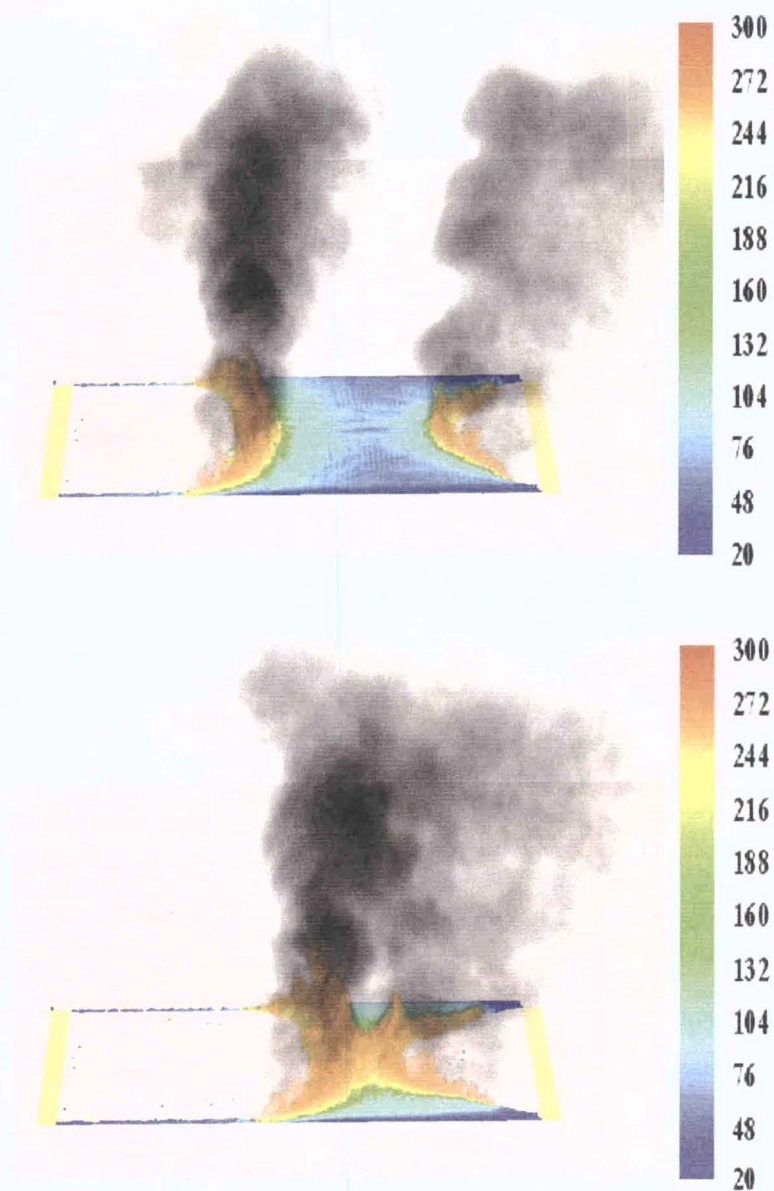
Fig. 2. Heat release rate (value > 135 \text{ kW/m}^3 ) and surface fuel temperature at time t = 153 \text{ s} and 163 \text{ s} (33 s and 43 s after the ignition of the two line fires), (10 m open wind speed: U_{10} = 1 \text{ m/s} ).
