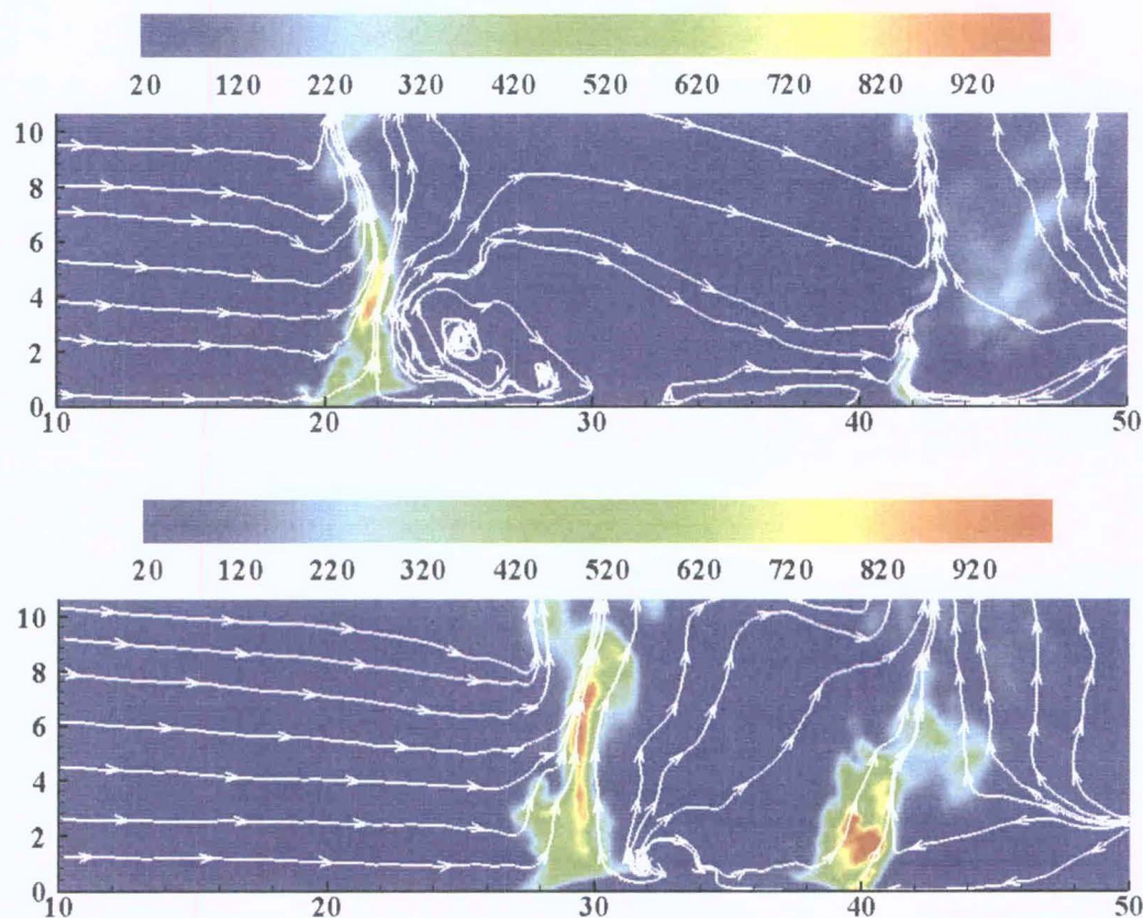
Fig. 3. Slide along a median plan of the temperature field and streamlines at time t = 153 s and 163 s ( 33 s and 43 s after the ignition of the two line fires in grassland; 10 m open wind speed: U_{10} = 1 m/s).
