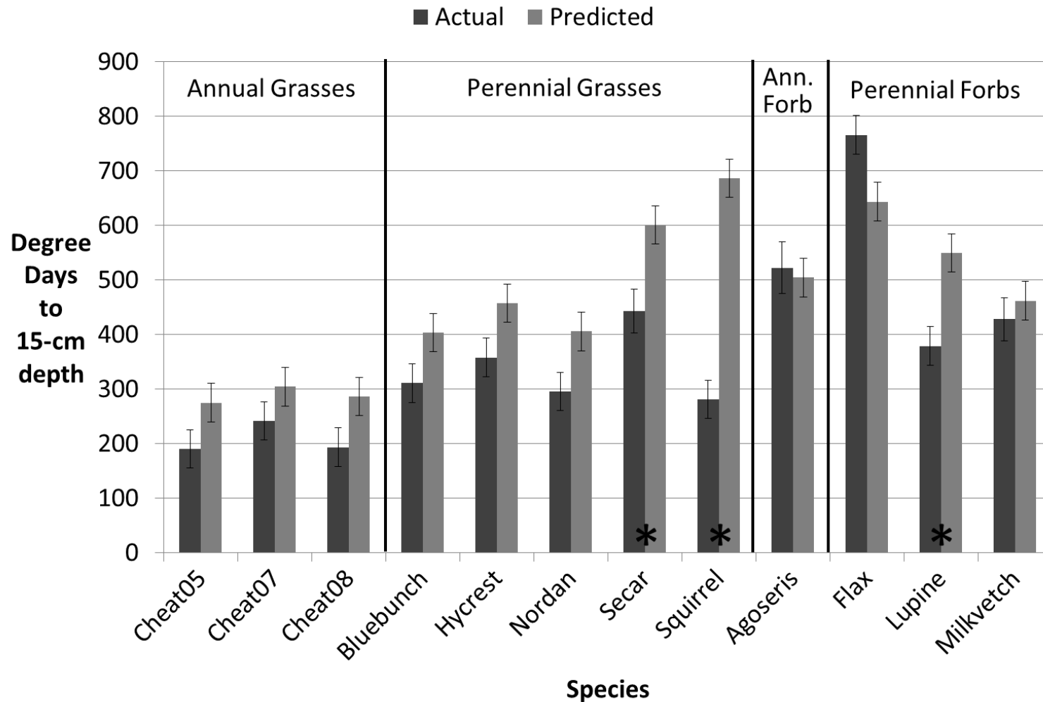
Figure 2. Actual versus predicted degree days to 15-cm root depth in soil for the growth chamber diurnal root trial 4-12°C. Asterisk (*) indicates significant difference at 95% confidence level.
