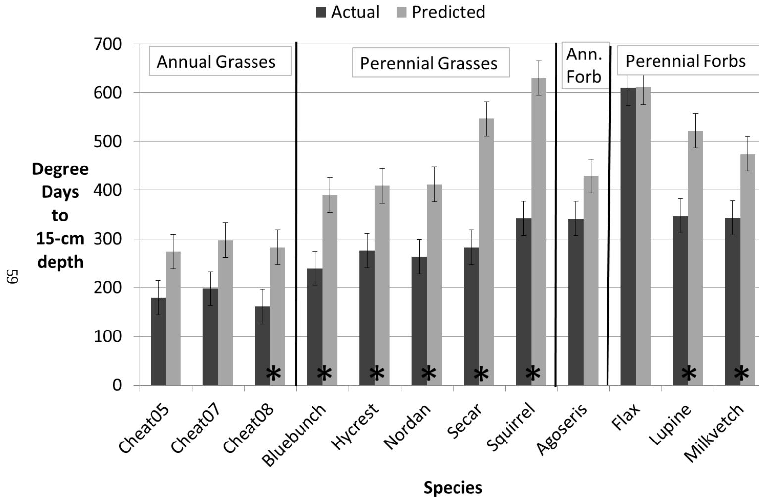
Figure 4. Actual verses predicted degree days to 15-cm root depth in soil for the growth chamber diurnal root trial 9-17°C. Asterisk (*) indicates significant difference at 95% confidence level.
