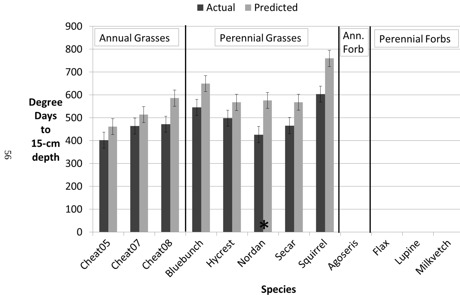
Figure 1. Actual verses predicted degree days to 15-cm root depth in sand for the growth chamber diurnal root trial 4-12°C. Asterisk (*) indicates significant difference at 95% confidence level.
