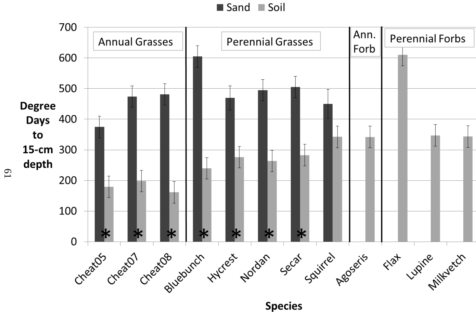
Figure 6. Actual sand versus soil degree days to 15-cm root depth for the growth chamber diurnal root trial 9-17°C. Asterisk (*) indicates significant difference at 95% confidence level.
