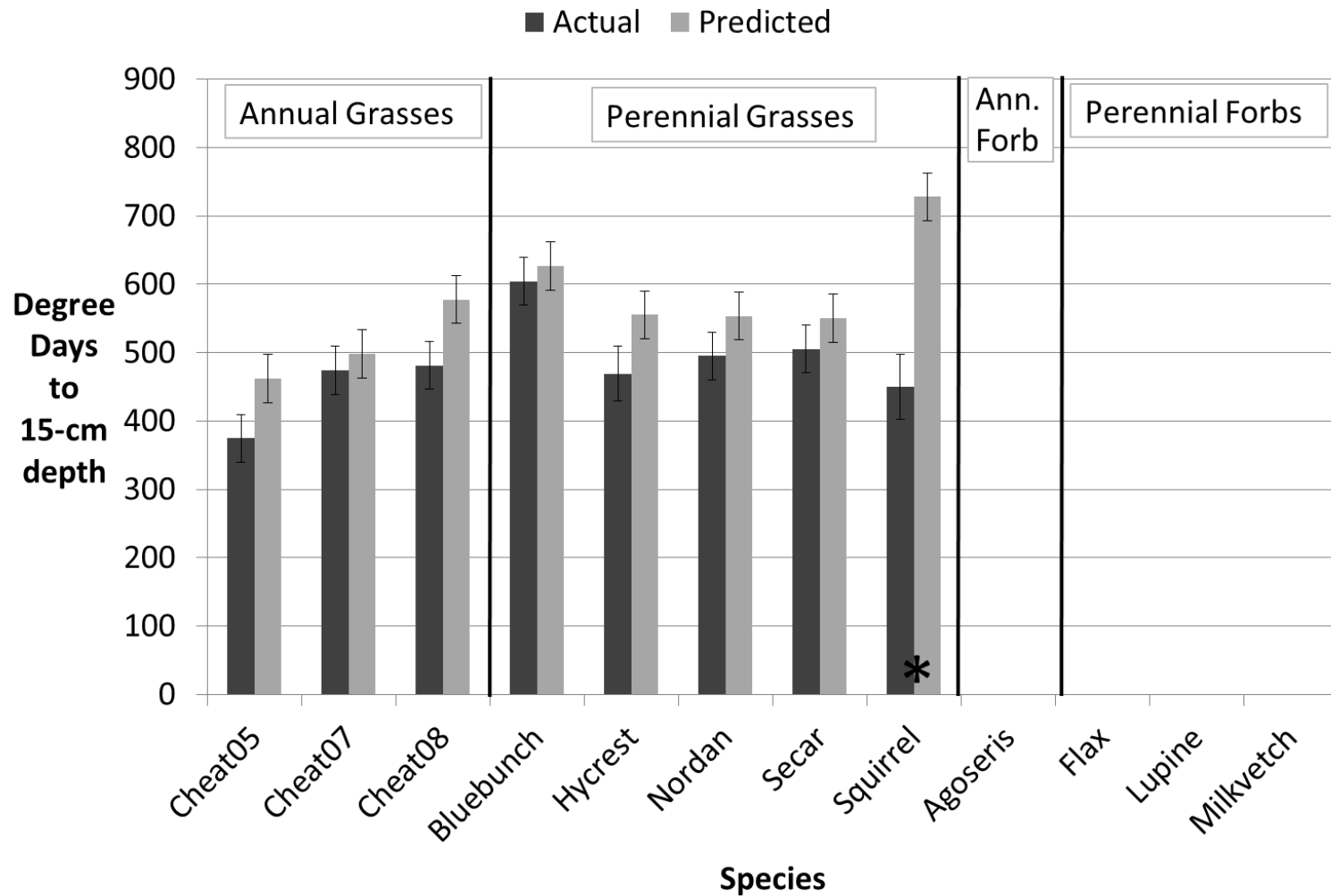
Figure 3. Actual verses predicted degree days to 15-cm root depth in sand for the growth chamber diurnal root trial 9-17°C. Asterisk (*) indicates significant difference at 95% confidence level.
