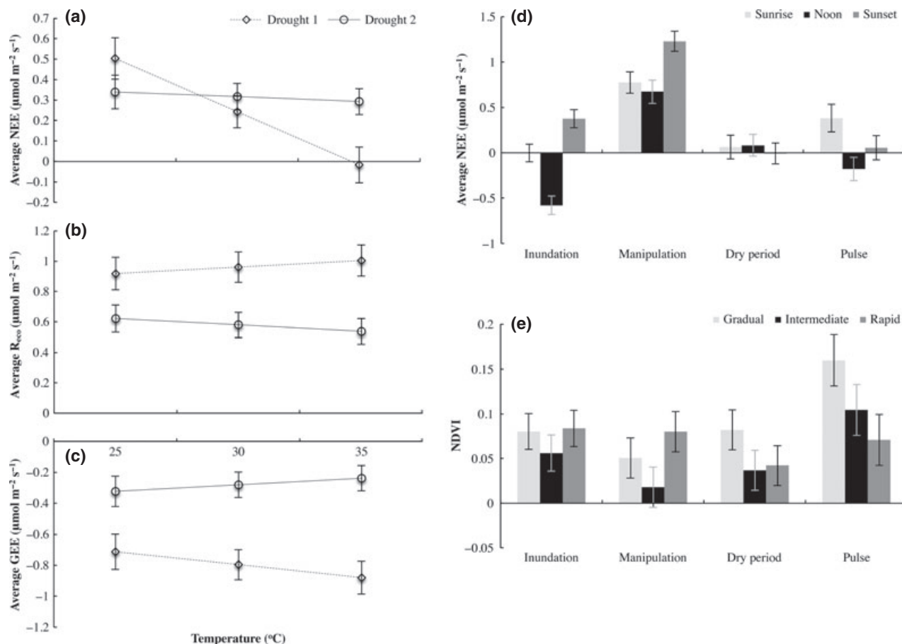
Fig. 2 Least square mean predicted values of the interactions between: (a) temperature and drought simulation for net ecosystem exchange (NEE), (b) R_{\text{eco}} , (c) gross ecosystem exchange (GEE), and (d) diurnal (sunrise, noon, and sunset) and experimental period (Inundation, manipulation, dry period, and pulse events) for NEE and (e) Normalized difference vegetation index (NDVI). Increasing temperatures resulted in higher fluxes in drought simulation 1 compared to drought simulation 2 (a–c). Net carbon uptake was greatest during midday measurement when monoliths were inundated and carbon release was greatest during manipulations (d–e). The chlorophyll content of the vegetation was highest for the gradual drought scenario during pulse events (d).
