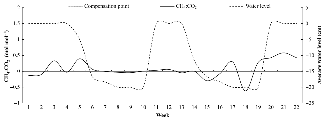
Fig. 3 Changes in average CH 4 to net CO 2 exchange over the study period in relation to average changes in water levels and the greenhouse carbon compensation point for 100 years (0.04). This system is a small source of carbon to the atmosphere due to the lack of recovery in net ecosystem exchange (NEE) during periods of inundation.
