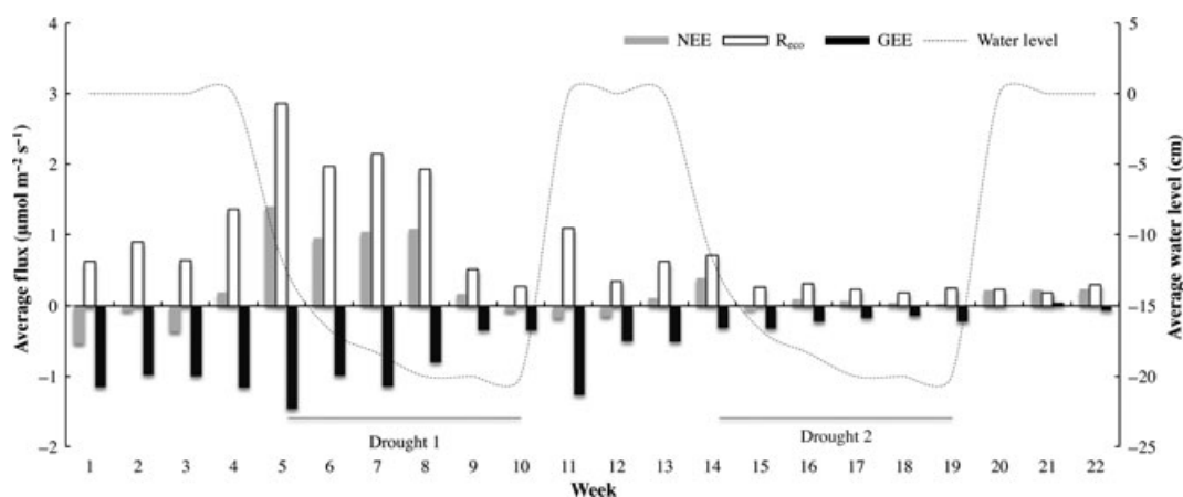
Fig. 1 Changes in average net ecosystem exchange (NEE), R_{eco} , and gross ecosystem exchange (GEE) over the study period in response to changes in water level for all drought scenarios. NEE and GEE were lowest (greater carbon uptake) during periods of inundation and highest (greater carbon release to the atmosphere) during drought simulations. R_{eco} increased during drought simulation up until water began limiting respiration rates.
