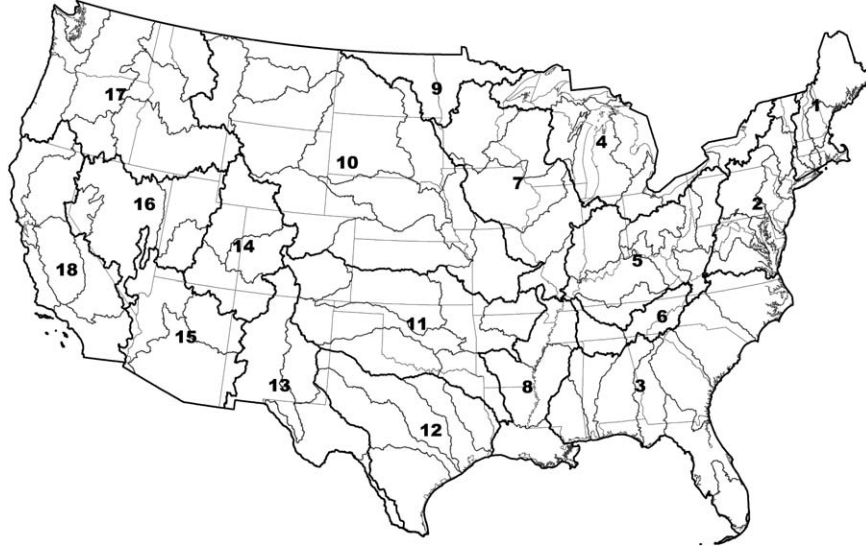
Figure 1. WRRs (numbered) and ASRs.
