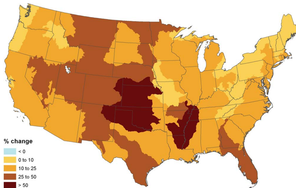
Figure 8. Change in ASR withdrawal from 2005 to 2060 attributable to climate change for the A1B scenario, multimodel average.
