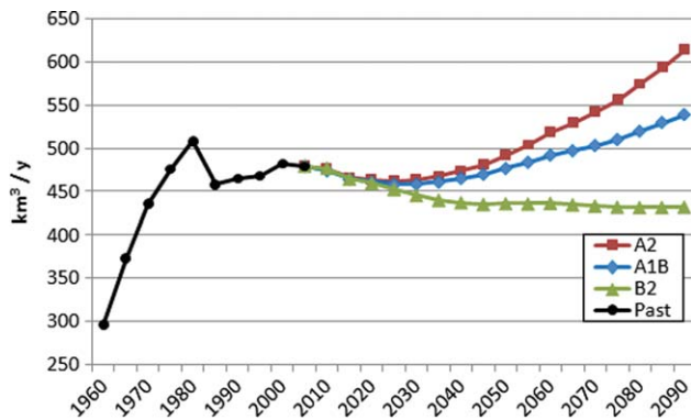
Figure 3. Past and projected annual water withdrawal in the U.S., given future population and income for three scenarios, no future change in climate.
