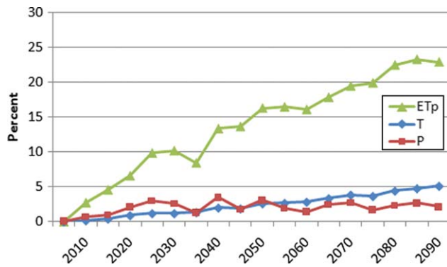
Figure 7. Trends in effects of climate change on projected total annual withdrawal in the U.S., averaged over the nine scenario-model combinations (percent change in withdrawal from a future with no climate change to a future with climate change caused by projected changes in potential evapotranspiration, temperature, and precipitation).
