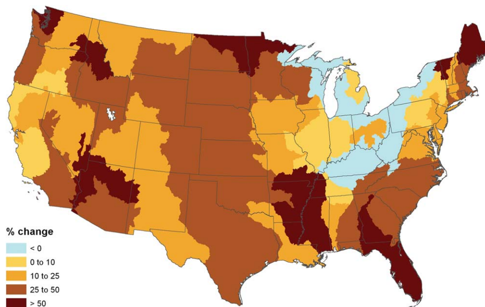
Figure 10. Change in ASR withdrawal from 2005 to 2060 for the A1B scenario, multimodel average.
