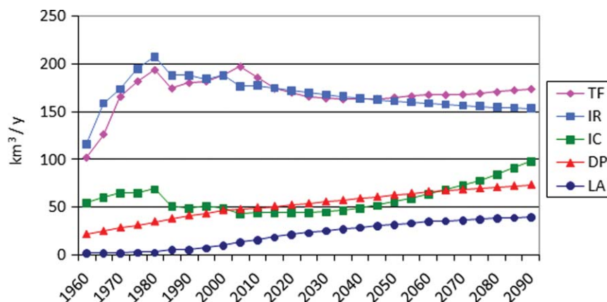
Figure 4. Past and projected annual withdrawal in the U.S. by water use sector, future population, and income of the A1B scenario, no future climate change (see Table 2 for sector definitions).
