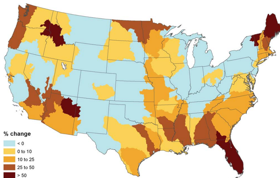
Figure 6. Change in ASR withdrawal from 2005 to 2060, given population and income of the A1B scenario, no future climate change.
