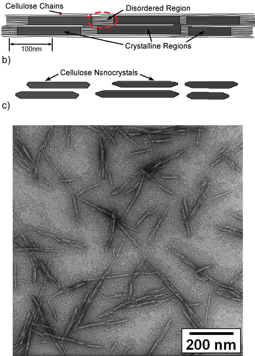
FIGURE 3-4 Cellulose nanocrystals. Top , Stacking of cellulose chains showing areas of “order” and “disorder.” During one type of cellulose nanomaterial extraction process that uses acid hydrolysis, the amorphous regions are preferentially dissolved and only the crystalline regions are left. Bottom , Transmission electron micrograph of cellulose nanocrystals produced by acid hydrolysis. SOURCE: Moon et al. 2011, used with permission.
