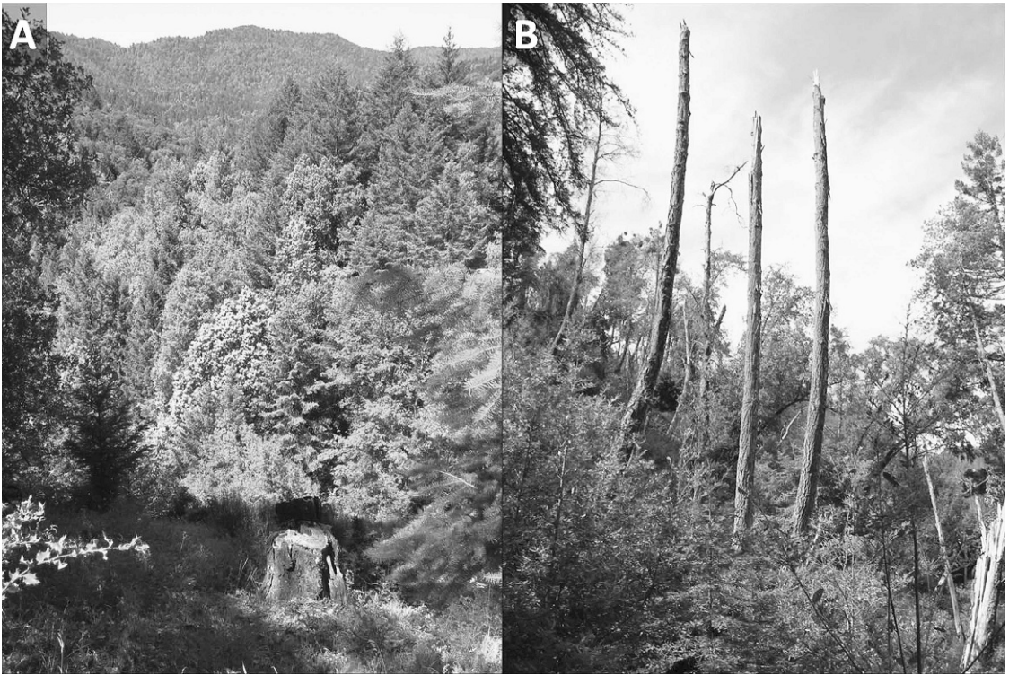
FIG. 2. Landscapes and stands that have not been invaded by Phytophthora ramorum (A) offer different opportunities and require different management approaches compared to invaded forests (B) when the goal is to retain tanoak and its associated flora and fauna. Variation in the likelihood of pathogen invasion into pathogen-free landscapes and stands is largely driven by proximity to pathogen invaded stands and community composition. Community composition can be manipulated to slow invasion and disease impacts. Disease impacted stands (e.g., B) require a host-centric management approach that avoids removal of surviving tanoak, protects potential genetically based resistance, and retains ecological functions and species obligate to tanoak. In both cases, successful conservation of tanoak will require continuous feedback between research and management to establish baselines, test hypotheses, and determine the efficacy of management actions.
