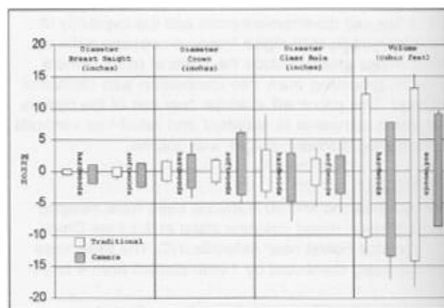
Figure 2—Errors for camera and standard methods for varying stem characteristics. The box indicates a 95 percent confidence interval about the mean (assuming normal distributions), and tails indicate the maximum and minimum observations.
