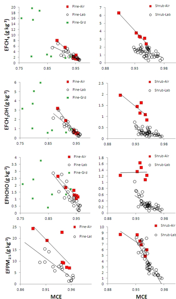
Fig. 2. Comparison of EF versus MCE from the lab and the field fires for smoldering compounds and \text{PM}_{2.5} for pine understory (left column) and semiarid shrubland (right column). The “Grd” (green symbols) indicate data for residual smoldering combustion provided for context (see text).
