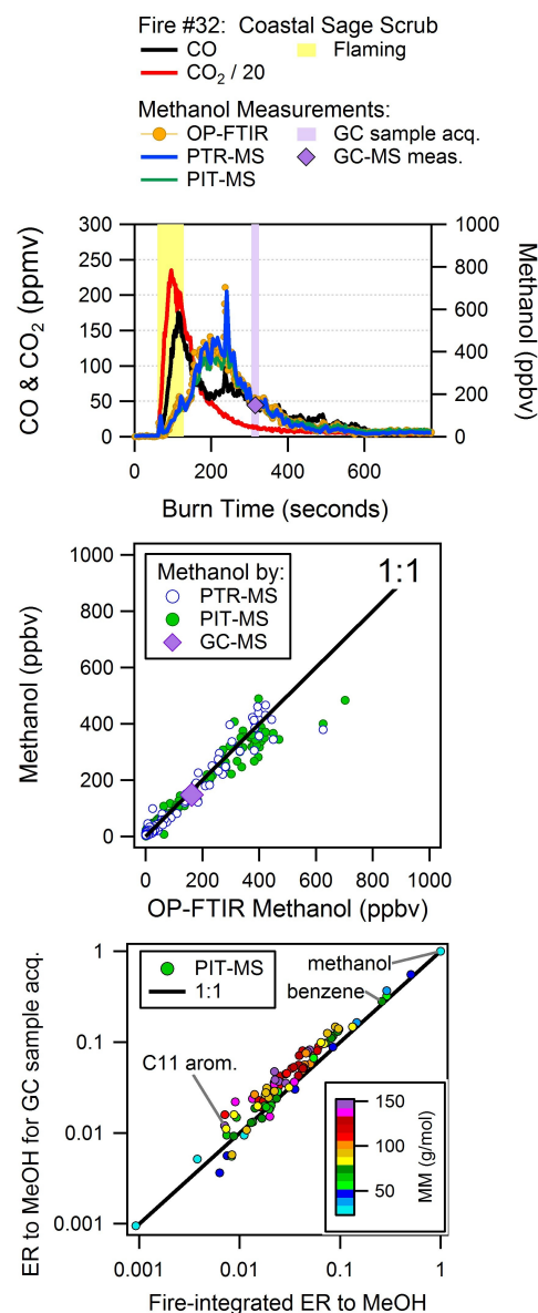
Fig. 1. (top) Time series for CO, \text{CO}_2 , and methanol for an example burn of coastal sage scrub (Fire #32). The yellow shading indicates the flaming-dominated period. The purple shading indicates the GC-MS sample acquisition time for this particular fire. (middle) A comparison of all other methanol measurements to the OP-FTIR methanol for Fire #32. (bottom) NMOC to methanol emission ratios (ER) as measured by the PIT-MS during the GC-MS sample acquisition time versus the ER determined by the PIT-MS during the entire fire for Fire #32 (see Sect. 2.2).
