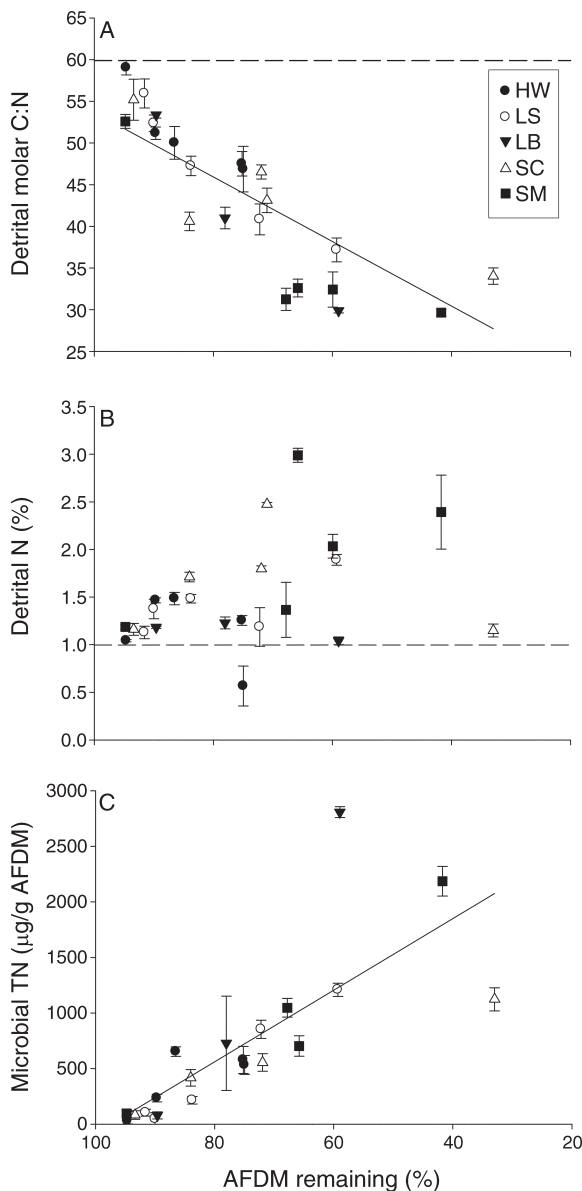
FIG. 3. Changes in detrital and microbial N content as a function of extent of decomposition. Error bars in panels (A) and (B) are \pm SE, while error bars in panel (C) are \pm 95\% confidence intervals. The dashed lines in panels (A) and (B) represent the condition of leaves before deployment, and solid lines are linear regressions including all sites with \text{C:N} = 0.387 \times \text{AFDM remaining} + 14.961 and microbial total N (TN) = -32.202 \times \text{AFDM remaining} + 3137.561 . Note that AFDM decreases from left to right along the x-axis. Detrital %N is expressed as a percentage of detrital AFDM.
