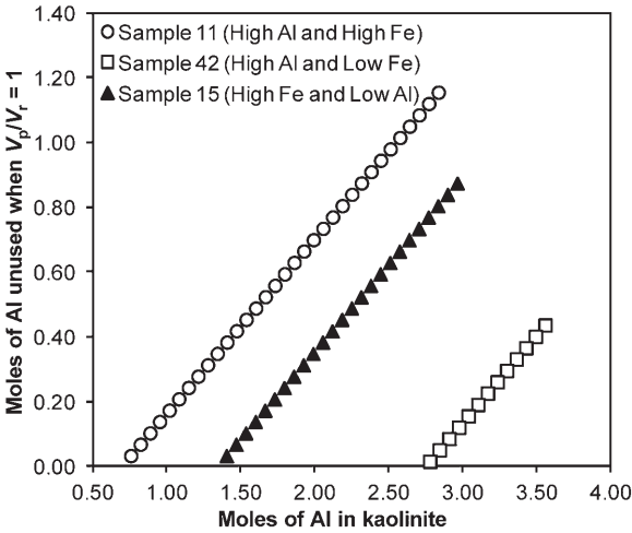
Figure 4. Relationship between Al stoichiometric coefficient of PSL kaolinite and the quantity of excess Al available for export from the almandine garnet-PSL microenvironment. Calculations (Table 4) based on almandine garnet data from Deer et al. (1997) (Table 2).
