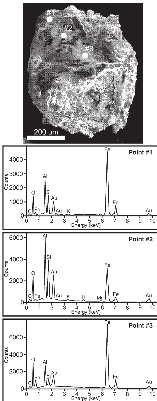
Figure 7. SEM-SEI image and EDS spectra of an Otto Formation garnet with surface layer hand picked from the regolith. Note the presence of Si in all spectra. Sample W34-6.
