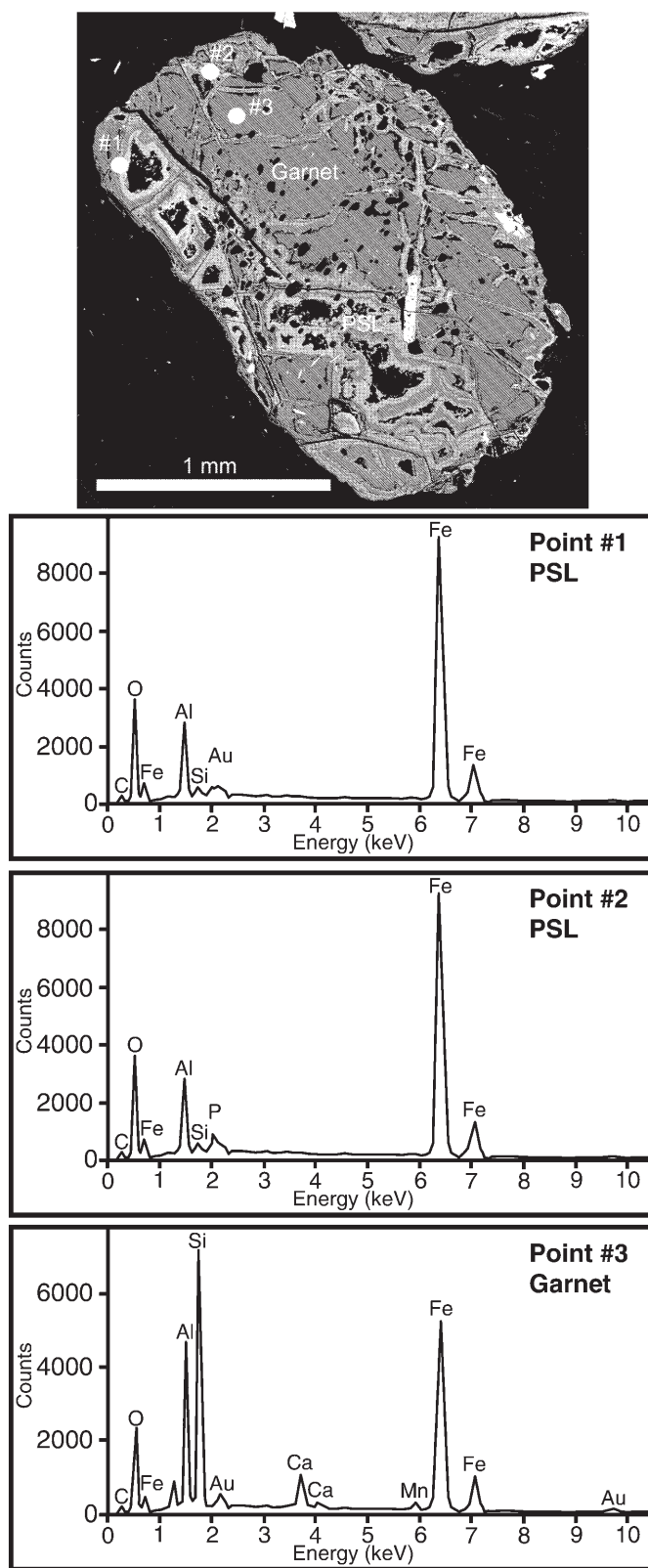
Figure 8. SEM-BEI image and EDS spectra of an Otto Formation garnet with surface layer. Points #1 and #2 are from the PSL and Point #3 is the unweathered garnet. Note the presence of Si in both PSL spectra. Sample W2-5.
