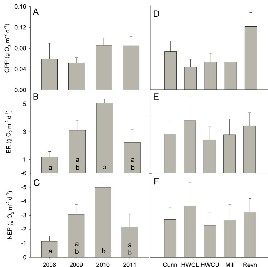
Figure 3. Metabolic parameters in Coweeta streams. Changes in gross primary production (GPP), ecosystem respiration (ER), and net ecosystem production (NEP) for low-order streams in Coweeta Hydrologic Laboratory over the years of the study (A–C) and in each stream (D–F). Error bars represent 1 SE of the mean, and different letters represent significant differences ( p < 0.05 ) based on Wilcoxon post-hoc multiple comparison tests.
