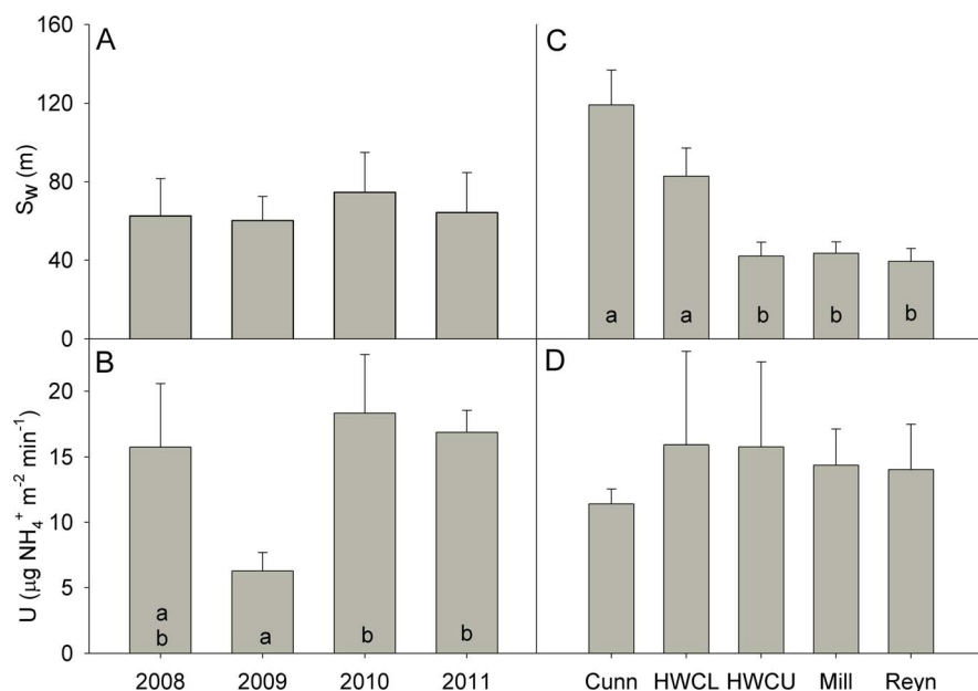
Figure 2. Nutrient uptake parameters in Coweeta streams. Changes in ammonium uptake length ( S_w ) and areal uptake ( U ) for low-order streams in Coweeta Hydrologic Laboratory over the years of the study (A–B) and in each stream (C–D). Error bars represent 1 SE of the mean, and different letters represent significant differences ( p < 0.05 ) based on Wilcoxon post-hoc multiple comparison tests. doi:10.1371/journal.pone.0061171.g002
