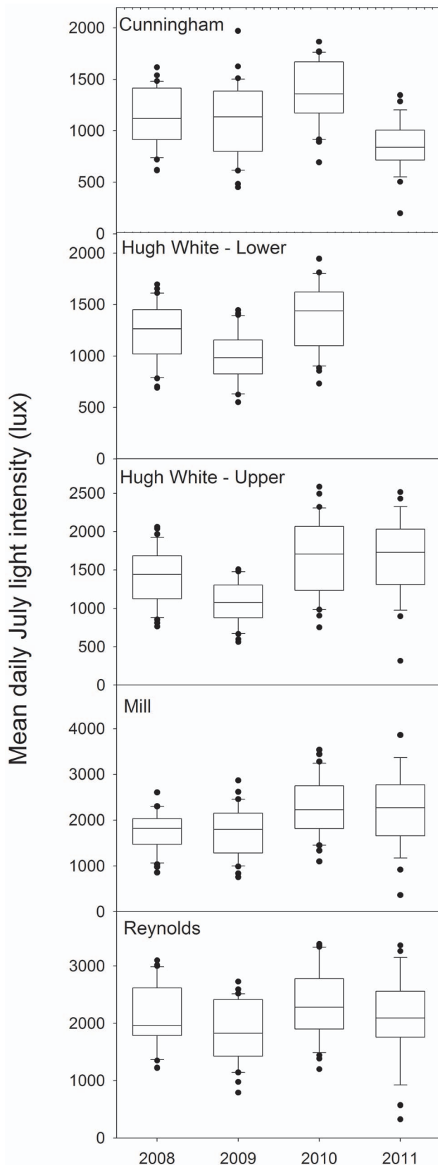
Figure 1. Light penetration in Coweeta streams. Distribution of July light intensities (lux) at the five study sites in Coweeta Hydrologic Laboratory over the course of the study. doi:10.1371/journal.pone.0061171.g001
