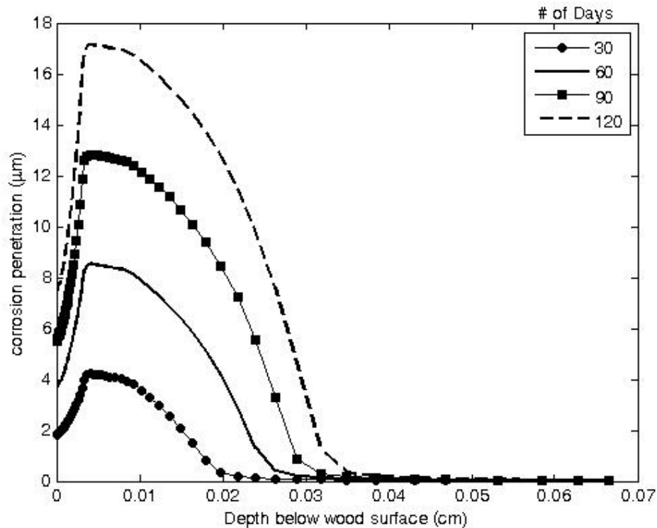
Figure 6: Simulation results of the amount of corrosion along the length of the fastener.
