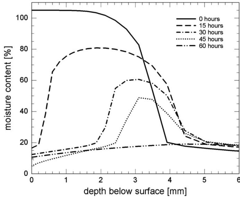
Figure 1: Moisture content profile after a rain event from 2D simulations conducted by Zelinka et al. 12 ; the different curves show how the profile changes with time after the rain stops. Note that the maximum depth of water ingress (~4 mm) is much less than the width of the specimen (~40 mm).
