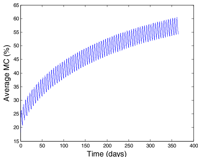
Figure 4: Average moisture content of the wood specimen with the default simulation parameters after 1 year of testing. The specimen continues to accumulate moisture.
