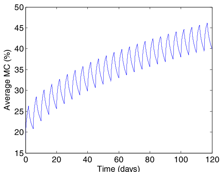
Figure 3: Average moisture content of the default simulation throughout the 120 test. Note the specimen is accumulating moisture throughout the test.
