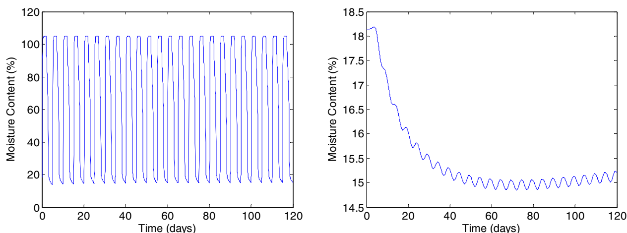
Figure 5: Moisture content 1mm below the surface receiving precipitation (left) and 70 mm below the surface, which corresponds to the bottom of the nail (right) for the default simulation.
