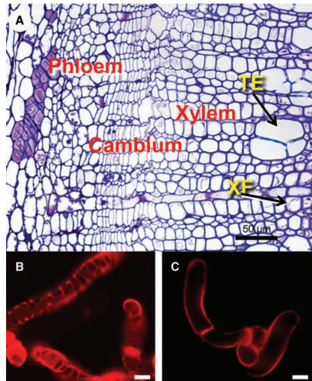
Figure 8. Xylem cells.
