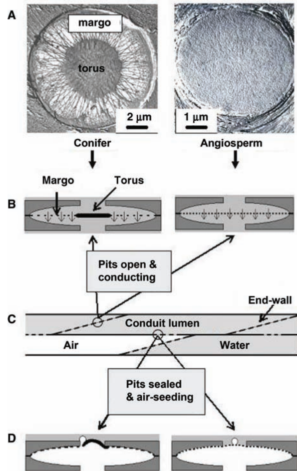
Figure 16. Structure and function of inter-conduit pits in conifer tracheids (left) and angiosperm vessels (right).
