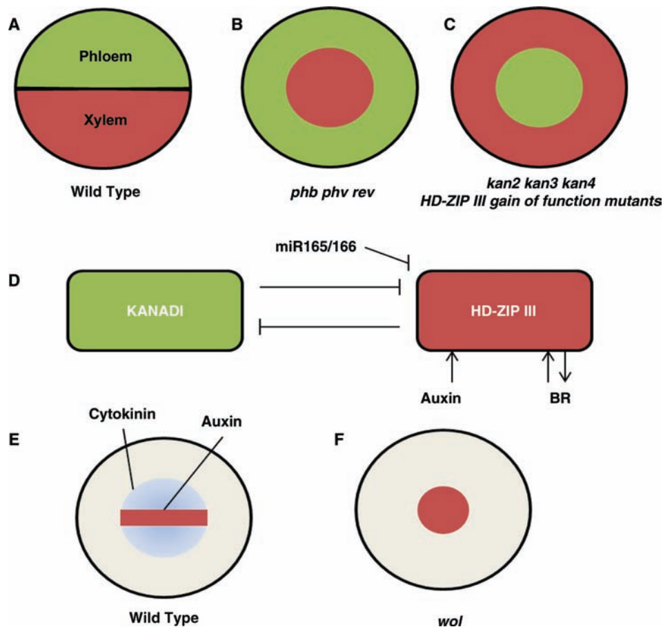
Figure 6. Vascular patterning is regulated by KANADI and Class III HD-ZIP genes and the phytohormones auxin and cytokinin.
