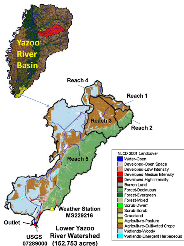
Fig. 2. Land use cover for the Lower Yazoo River Watershed.
