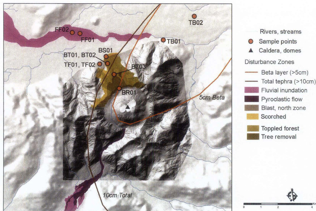
FIG. 2. Map of zones and plot (circle) and observation (triangle) locations within about 5 km of the volcano. The north flank blast zone delineations are from Major et al. (2013, this volume) plus a small photo-interpreted area to the north. The DEM for the central, high-resolution part of image is compiled from LIDAR surveys conducted by Digimaps Chile between 15 October and 7 December 2009 and provided by the Regional Government of Los Lagos region; see Major et al. (2013, this volume) for further details.
