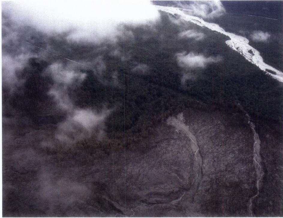
FIG. 5. Oblique aerial view of north flank with toppled-tree and scorch zones in foreground and Rayas River in upper right, looking to the northwest. This 6 June 2008 view shows the narrow scorch zone with foliage (brown) still on the trees between the toppled-tree zone (lower part of photo) and living forest (green trees in upper part of photo) (photo: A. Lockhart, USGS).
