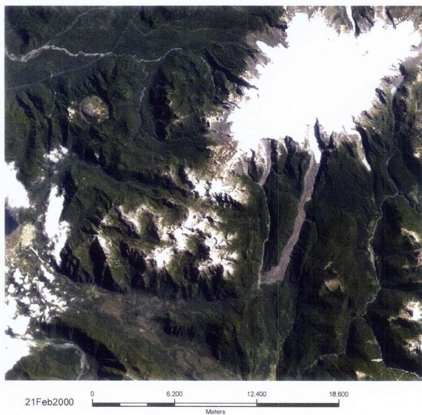
FIG. 3. True-color satellite image of Chaitén, 21 February 2000 (Source: NASA Earth Observatory, http://earthobservatory.nasa.gov/NaturalHazards/view.php?id=19894 ).
