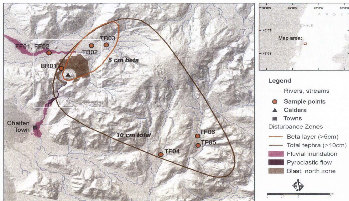
FIG. 1. Map of study area, disturbance zones, sample plots (circles), observation points (triangles), and disturbance zones within several 10s of km of Chaitén volcano. Note that additional sample plot and observation point locations are shown on figure 2.
