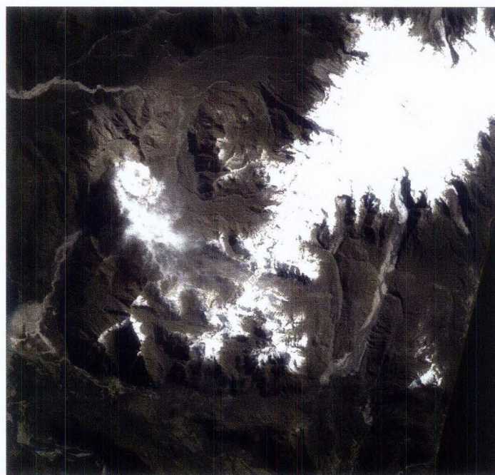
FIG. 3. True-color satellite image of Chaitén, 21 February 2000 (Source: NASA Earth Observatory, http://earthobservatory.nasa.gov/NaturalHazards/view.php?id=19894 ).
