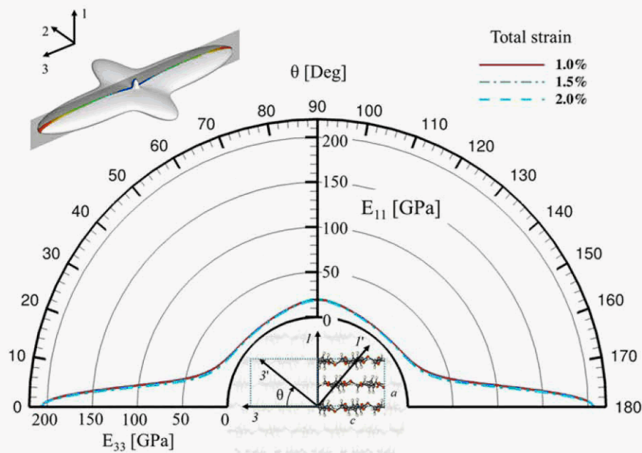
Fig. 5 Angular variation of the longitudinal Young's modulus ( E_A ) within the 1–3 plane for applied strains of 1.0, 1.5, and 2.0 %. The 2-axis (perpendicular to the page) is considered to be the rotation axis: the value of the longitudinal modulus for a given direction can be read directly from the figure by defining a straight line from the origin to the desired angle. It is important
