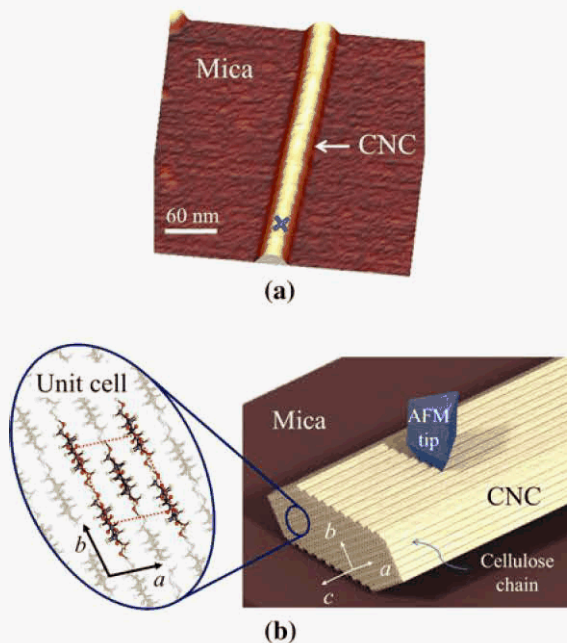
Fig. 1 a Atomic force microscope topography image of a tunicate CNC showing its rod-like shape (on a mica substrate) (Wager et al. 2011). The blue cross near the bottom of the figure denotes a location for AFM tip indentation. b Schematic of a CNC particle during AFM indentation for illustration purposes. Here, the cellulose chains are represented as straight ribbons, and the crystallographic directions indicated as a , b and c . The inset shows details of the layered cellulose structure where red spheres denote oxygen ions, gray spheres represent carbon ions and white spheres represent hydrogen ions. The red dotted lines indicate the repeating unit cell. (Color figure online)
