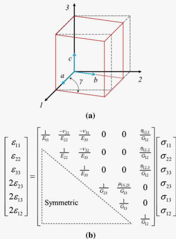
Fig. 3 a Schematic representation of the cellulose I_8 monoclinic ( P2_1 ) unit cell aligned with the Cartesian coordinate system used in this study (red solid lines). A rectangular prism cell (black dashed lines) is used to help visualize the orthogonality between the a - c and b - c axes, highlighting the non-orthogonal relationship between a and b . b Relationship between the strain and stress vectors via S_{ij} (Jones 1975) ( \varepsilon_{ij} = S_{ijkl} \sigma_{kl} ) for the P2_1 cellulose I_8 unit cell. E_{ii} is the Young's modulus in the i -direction, G_{ij} is the shear modulus in the i - j plane, \nu_{ij} is the Poisson's ratio which quantifies the contraction in the j -direction due to uniaxial loading in the i -direction, \eta_{ij,k} are the coefficients of mutual influence of the first kind which characterize normal strain in the k -direction due to shear stress in the i - j plane, and \mu_{ij,k} are Chentsov's coefficients which characterize shear strain in the k -plane due to shear stress in the i - j plane. (Color figure online)
