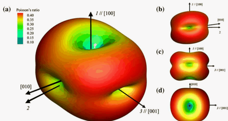
Fig. 7 Average Poisson's ratio \bar{\nu}_{1'} surfaces for cellulose I_k computed using Eq. 1 based on S_y for 1.0 % of total deformation in the Le Page and Saxe method (Le Page and Saxe 2002). Each point on the surface represents the magnitude of Poisson's ratio in the direction of a vector from the origin to that point. The
