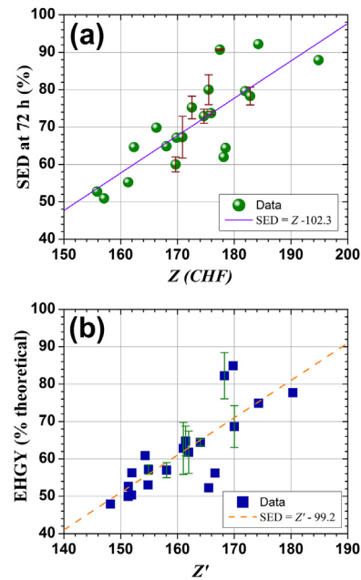
Fig. 6 – Correlations of substrate enzymatic digestibility (SED) and enzymatic hydrolysis glucose yield (EHGY) with combined factors of delignification and carbohydrate loss Z (CHF) and Z' , respectively. (a) SED with Z (CHF); (b) EHGY with Z' .
