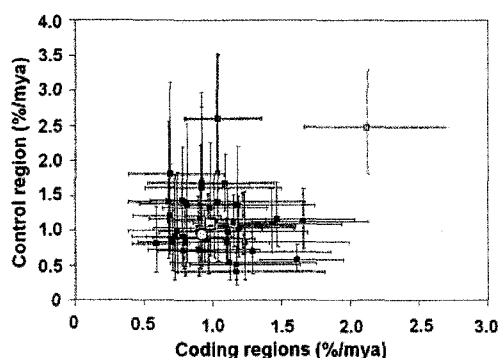
FIG. 4. —CR and protein-coding region lineage specific substitution rates for the 42 cetacean species included in this study. Error bars associated with points indicate the 95% HPD associated with each species. The sperm whale is shown in blue, the Franciscana ( Pontoporia blainvillei ) in green and the killer whale ( Orcinus orca ) in red. The median odontocete rates are shown in the yellow square, the median mysticete rates in the yellow circle.
