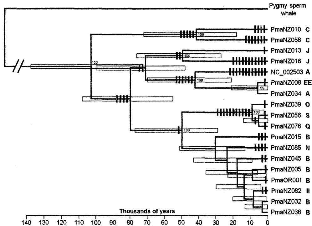
FIG. 1. —Bayesian phylogenetic reconstructions of the relationship between the 17 sperm whale mitogenomes in this study based on protein-coding genes (10,815 bp), including the NCBI GenBank sample, NC_002503 (Arnason et al. 2000). Terminal taxa are labeled by their individual sample codes and CR haplotypes (400 bp) are listed in bold after sample codes. Clades with more than 95% posterior probability are indicated on the tree, and 95% HPD intervals for node ages are shown by the horizontal blue boxes. Parsimony-inferred character changes (using Mesquite v2.75; Maddison and Maddison 2011) in the protein-coding regions are shown by black cross bars. Inferred character changes in the 400 bp region of the CR used to define haplotypes are shown in gray. Homoplastic characters are shown in shades of blue for the protein-coding region (two sites requiring two changes each), and in shades of red for the CR (also two sites requiring two changes each). Consistency Indices: 0.9722 for protein-coding regions and 0.8333 for CR. Retention Indices: 0.9565 for protein-coding regions and 0.8333 for CR.
