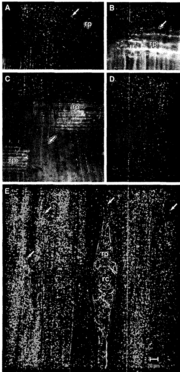
Fig. 2. Movement of aqueous acid fuchsin in the sapwood of Douglas-fir under a radial pressure gradient. Conducting cells are stained in red in panels A–D, images are of frozen radial sections and wide-field cryo-fluorescence microscopy. (A) General view of a radial section showing movement of the dye in ray parenchyma (rp) but not in ray tracheids (rt) (arrow). (B) Detail of the same section shown in panel (A). (C) Movement of the dye in axial tracheids and acid fuchsin bound to cell walls (red color, arrow). (D) Stained earlywood and unstained latewood and that the radial distribution of the dye is limited because of a higher resistance to the radial apoplastic flow at growth-ring boundaries and latewood tracheids. Panel E is a freeze-dried tangential section imaged with confocal microscopy that was cut 2–3 mm apart from the stained axial tracheids and shows that the dye is transported through ray parenchyma but did not fill ray tracheids and resin canals.
