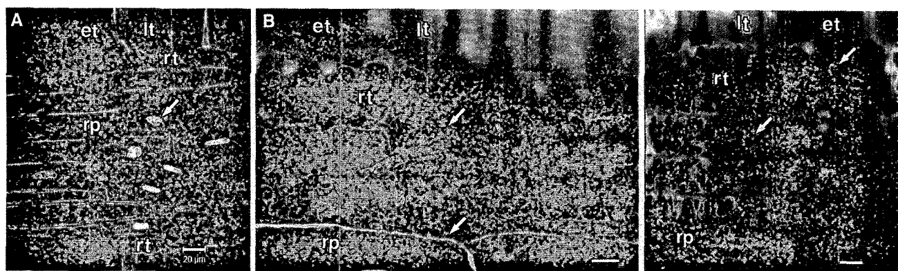
Fig. 3. Structure of xylem rays in radial sections of sapwood visualized by confocal microscopy. (A) Ray tracheids (rt), ray parenchyma (rp), and boundary between earlywood tracheids (et) and latewood tracheids (lt) in Douglas-fir. Ray parenchyma cells are thick-walled with nuclei and protoplasts. (B) Thin-walled, nonlignified ray parenchyma and thick-walled ray tracheids in ponderosa pine. The upper arrow shows ray tracheid to ray tracheid bordered pits and the lower arrow shows pits between ray tracheids and ray parenchyma. (C) Lodgepole pine with thick-walled ray parenchyma and short and thick-walled ray tracheids. The upper arrow shows earlywood tracheid to ray tracheid bordered pits (outer side of the earlywood tracheid cell wall); lower arrow shows ray tracheid-to-latewood tracheid bordered pits (inner side of the ray tracheid wall).
