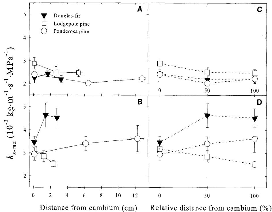
Fig. 1. Sapwood radial conductivities of east side (upper panels) and west side (lower panels) for (list the species). Panels A and B represent radial conductivities in relation to absolute sapwood depths; panels C and D represent conductivities at relative sapwood depths. Error bars represent one standard error ( N = 12 ).
