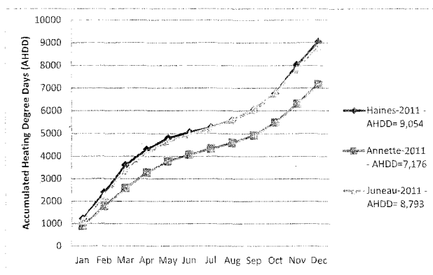
Figure 1.—Accumulated heating degree days for three locations in southeast Alaska.
