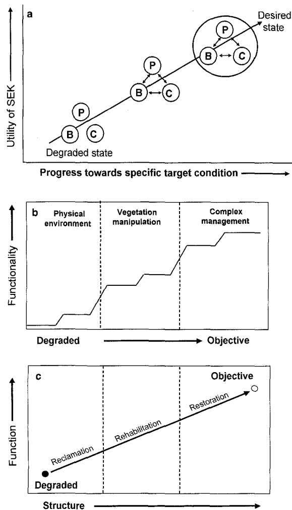
Fig. 11 Framework for integrating soil ecological knowledge (SEK) with theoretical models of ecosystem restoration. (a) When sites are heavily degraded, some improvement in soil function may be achieved by manipulations of either the chemical (C), physical (P), or biological (B) attributes of the soil. For greater progress toward a target condition, however, an increase in the degree of complex SEK is required, and there are more complex interactions among P, C, and B attributes. To achieve the desired state of restoration requires very high level understanding of P, C, and B processes. (b) Physical, biological, and management thresholds that must be overcome if restoration is to be successful. Hypothesis 11 is consistent with the likelihood of faster restoration of functionality with respect to physical processes such as hydrologic flow and slower restoration of biogeochemical processes. (c) The integral relationship between structural and functional attributes in ecosystem restoration (figure reproduced with permission from Heneghan et al. , 2008).
