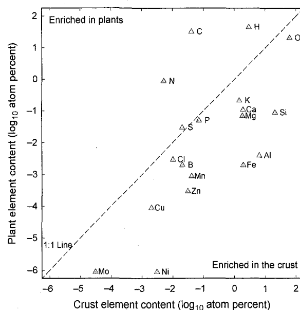
Fig. 2 Abundance of elements in Earth's crust compared with abundance in plant tissues. Data compiled by J. R. Leake.
