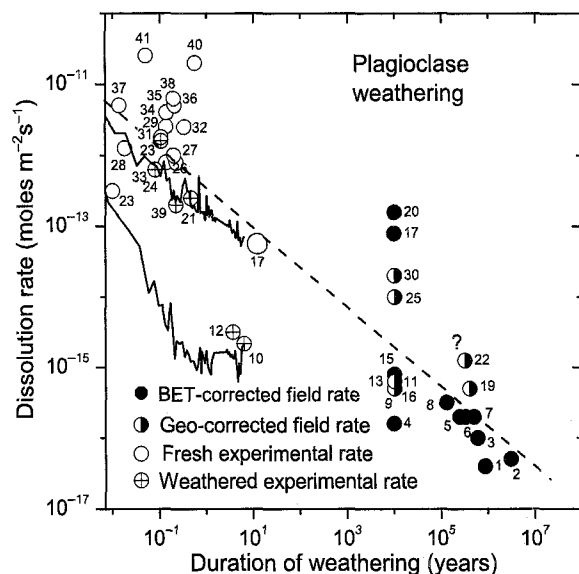
Fig. 6 A plot showing how the rate of dissolution of plagioclase feldspar varies as a function of the duration of observation (plotted in years on the x-axis). Measurements of this rate in the laboratory are orders of magnitude faster than the rates estimated in natural systems. Filled symbols represent rates measured in the field that have been normalized by the surface area of the feldspar measured by BET analysis. Half-filled data denote field rates corrected for geometric surface area. Open symbols represent rates measured in the laboratory for freshly ground unaltered samples; open symbols with crosses delineate laboratory rates measured for samples that were previously weathered in the field. The dashed line is a regression fit to the data. Solid lines indicate the measured laboratory rate of dissolution of pristine or previously weathered Panola granite as a function of time. Figure revised from the original publication: references for original data as indicated by numbers are found in the original reference (White & Brantley, 2003). Many explanations have been advanced for why rates vary with duration of observation, including the effects of changing soil structure with time, changing mineral surface chemistry with time, changing chemical affinity with time, the effects of biota, inadequacies in measurement of surface area, hydrologic factors, clay precipitation effects, etc.
