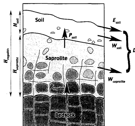
Fig. 4 Schematic showing regolith with thickness H_{\text{regolith}} (here equal to the combined thickness of the soil, H_{\text{soil}} , and saprolite, H_{\text{saprolite}} ) overlying unweathered parent material (labeled bedrock). Upward arrows denote fluxes of solid Earth materials across horizons; diagonal arrows denote fluxes out of the system. Chemical and physical weathering of parent material results in a flux of 'fresh' minerals into the regolith ( P_{\text{regolith}} ). Chemical denudation in saprolite ( W_{\text{saprolite}} ) prepares it for conversion into soil ( P_{\text{soil}} ). Physical and chemical denudation of soil ( E_{\text{soil}} and W_{\text{soil}} , respectively) removes it from the landscape. The sum of the denudational fluxes is the total denudation rate ( D ). Aeolian fluxes (not shown) may be an important additional source of mass in the CZ. Adapted from Riebe et al. (2003, 2004) and Dixon et al. (2009).
