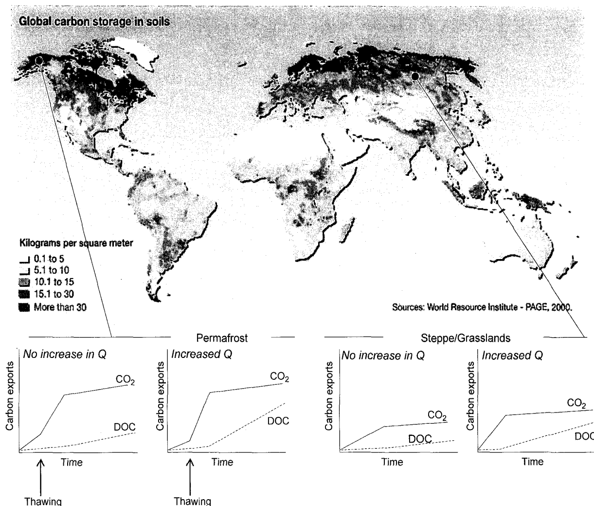
Fig. 7 Predictions of carbon export ( \text{CO}_2 and DOC) under a warming climate, with and without increases in discharge ( Q ). The two examples chosen are from northern latitudes which are expected to see the largest temperature increases. The difference in magnitude of the carbon exports is meant to reflect the difference in carbon storage between the regions. There are a variety of factors affecting carbon exports including those that affect net primary productivity and therefore total carbon stocks (e.g. climate, fertility, species composition) and those that affect the decomposition and export of those carbon stocks (e.g. temperature, water, substrate quality, oxygen). Base map is from the UNEP/GRID-Arendal Maps and Graphics Library (2009).
