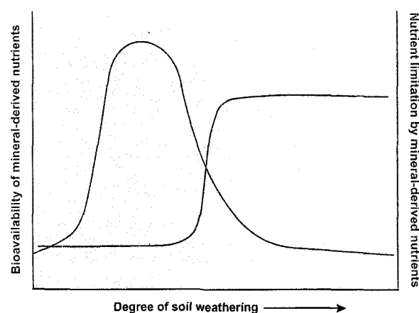
Fig. 3 A conceptual figure illustrating the hypothesized shift in the relationship between weathering and the biosphere for stable landscapes as discussed in Hypothesis 3. Soon after biota become established at a given location, the bio-availability of mineral-derived nutrients increases due to biotic stimulation of chemical weathering rates (see Fig. 1). Over time, as the degree of soil weathering progresses and nutrients are lost at a slow rate due to leakage from the system, biotic demand will eventually exceed the supply of mineral-derived nutrients, causing the system to shift into a state of nutrient limitation.
