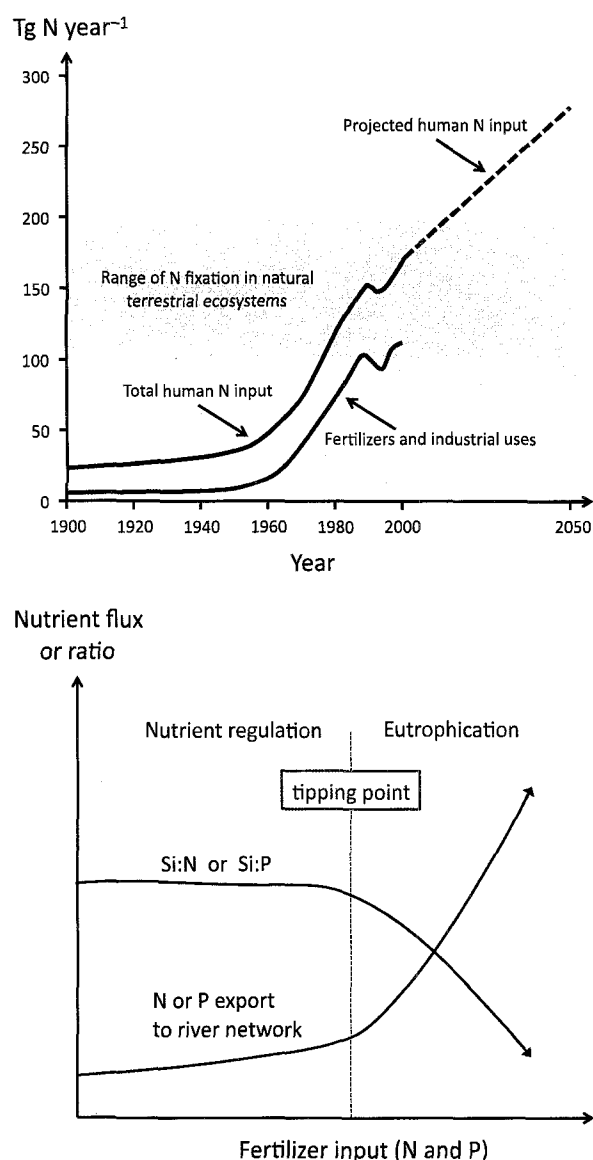
Fig. 12 Hypothetical response (lower figure) in buffering of nutrients by CZ processes as anthropogenic inputs of nitrogen (N) and phosphorus (P) via fertilizer application are increased (upper figure). At relatively low fertilizer loadings, processes such as denitrification that eliminate or processes such as sorption or plant uptake that retain N and P can limit the export fluxes from the soil environment. Beyond a threshold in fertilizer application, however, the natural buffering capacity of the soil is exceeded and there is a rapid transfer of bioavailable N and P to the stream network. If the export of bioavailable silicon (Si), primarily produced by chemical weathering of silicate minerals, remains constant, then the increase in N and P export fluxes is also accompanied by a drop in the Si:N and Si:P ratios. Both the absolute and relative changes in nutrient fluxes as the tipping point is crossed may cause significant downstream damage to in-stream ecosystems, freshwater reservoirs, and the coastal zone (Rabalais, 2002). Upper figure reproduced with permission from the Millenium Ecosystem Assessment (2005).
