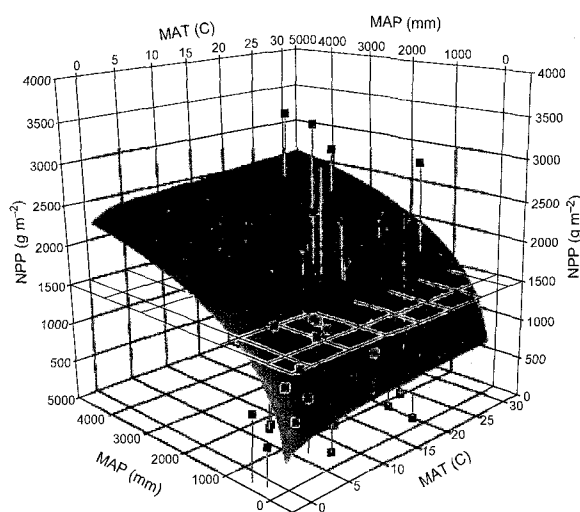
Fig. 5 A diagram illustrating the relationship between net primary production (NPP, grams of plant matter per square meter of land area), vs. mean annual precipitation (MAP, mm year -1 ) and mean annual temperature (MAT, °C). Individual data points are shown as black cubes. A multivariable regression model used to fit the data is illustrated as a smooth surface. Data from Lieth (1973), figure made by R. Amundson.
