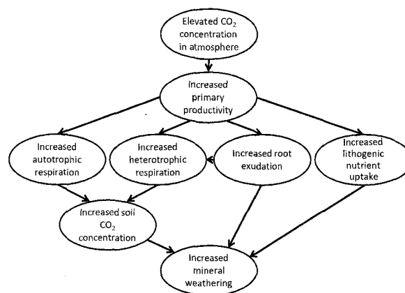
Fig. 8 Conceptual diagram for Hypothesis 8 that reflects a hypothesized relationship between elevated CO 2 in the atmosphere and rate and extent of mineral weathering. Length of the arrows and size of the pools do not indicate magnitude of the response or the reservoirs, as these are largely unknown, especially in different ecosystem types.
