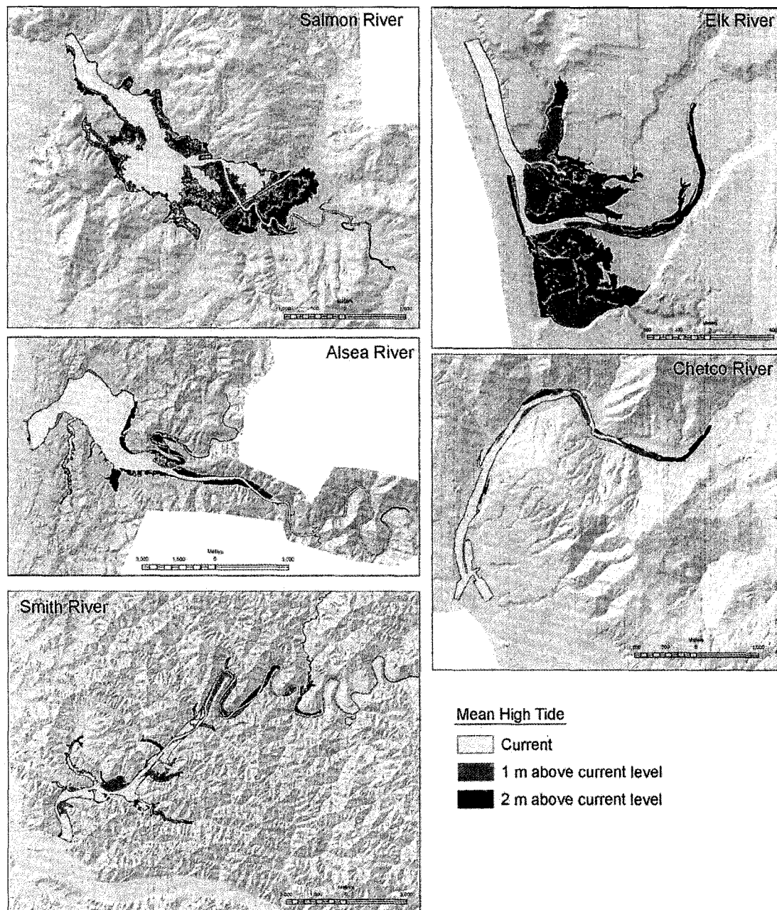
Fig. 5 Estimated estuary margin at current mean high tide, with a 1-m increase in mean sea-level, and with a 2-m increase in mean sea-level for: Salmon River, Alsea River, Smith River, Elk River, and the Chetco River
