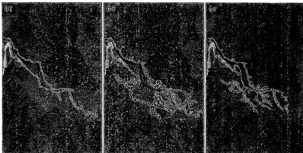
Fig. 4 Difference in baseline-current mean high-tide contour among: a 10-m digital elevation models (DEM), b LiDAR flown without considering tide level (coast-wide LiDAR), and c LiDAR flown
