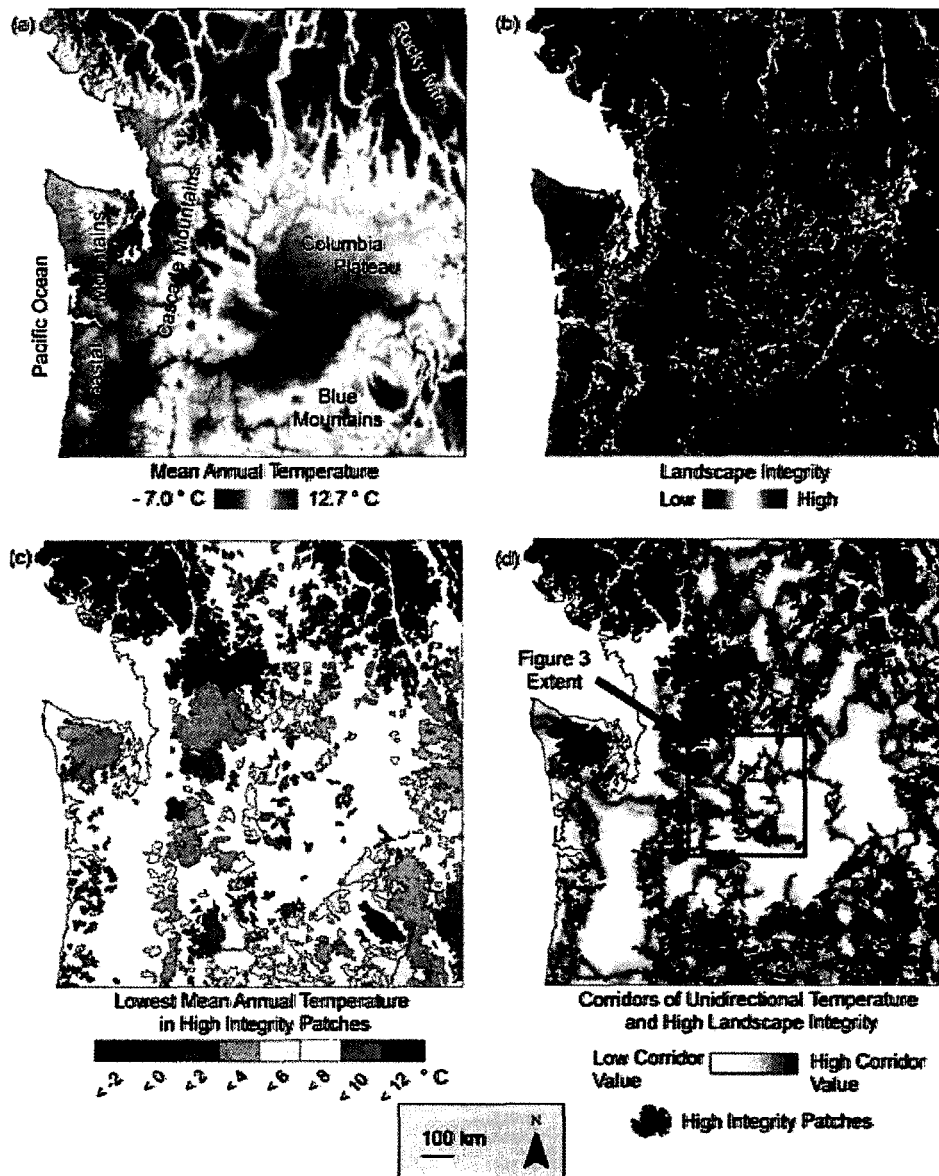
Figure 2. Data used in our climate corridor model included (a) a mean of mean annual temperatures from 1971 to 2000 and (b) a landscape-integrity index (a metric of naturalness that incorporate data on urban areas, distance to roads, agriculture, and other land uses).
