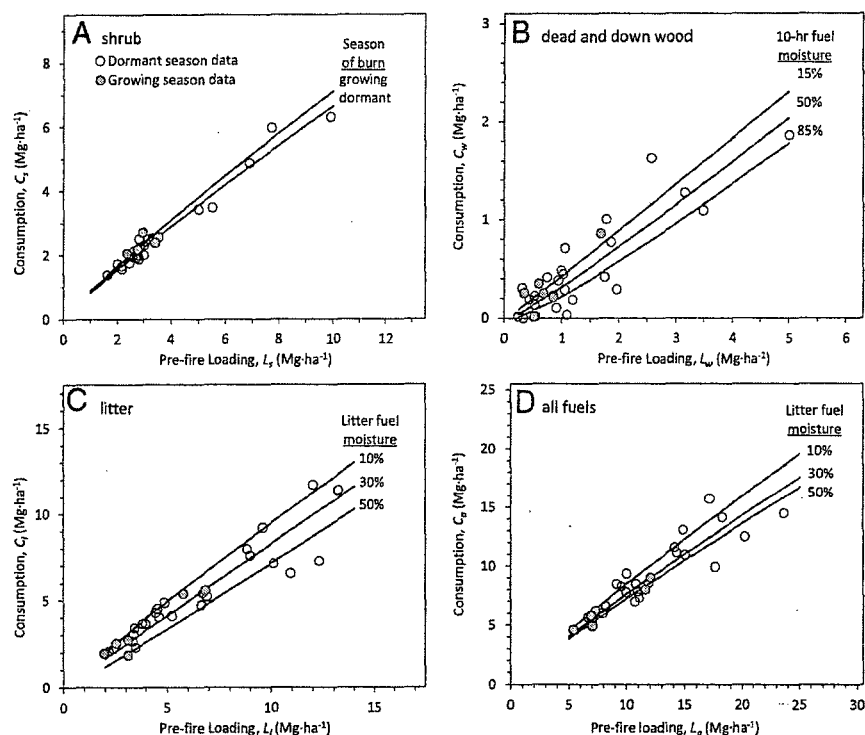
Figure 3. Multiple linear regression models showing: A) shrub consumption (including saw palmetto) as a function of prefire shrub loading and season of burn; B) dead and down woody fuel consumption as a function of prefire woody fuel loading for a range of values of 10-hour woody fuel moisture; C) litter consumption as a function of prefire litter loading for a range of values of litter fuel moisture; and D) total aboveground biomass consumption as a function of total aboveground prefire loading for a range of values of litter fuel moisture for pine flatwoods ecosystems.
