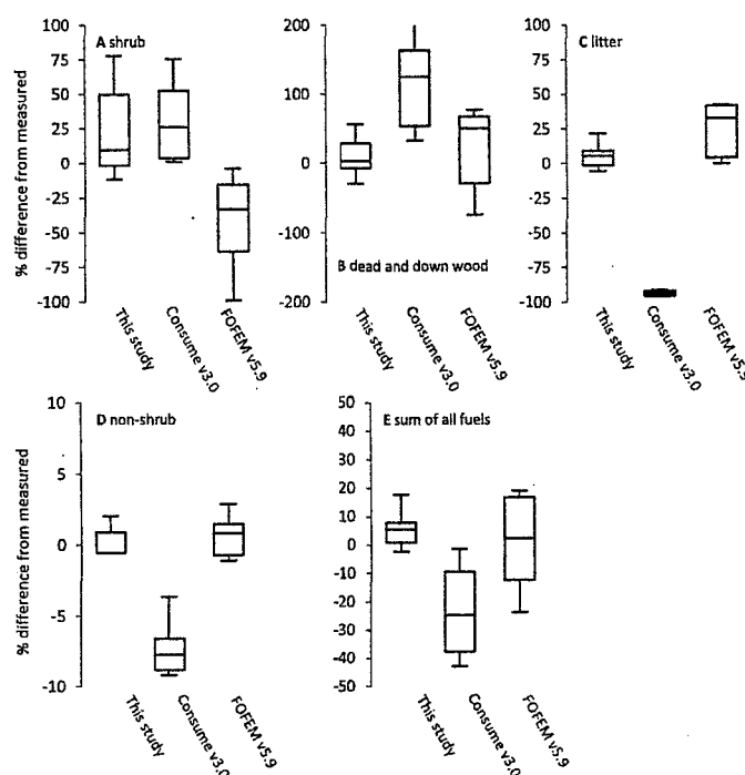
Figure 4. Difference from measured fuel consumption for predictions made with FOFEM 5.9, Consume 3.0, and the models reported in this study. Measured prefire fuel loading, day-of-burn fuel moisture, and fuel consumption are reported in Table 9.
