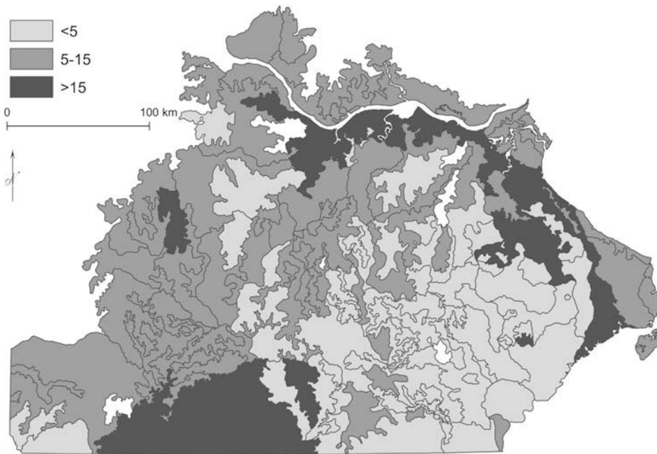
Figure 4. Increased percent composition of eastern redcedar in contemporary forests compared to historical forests (percent eastern redcedar in contemporary forests—percent eastern redcedar in historical forests; tree DBH \geq 12.7 cm).
