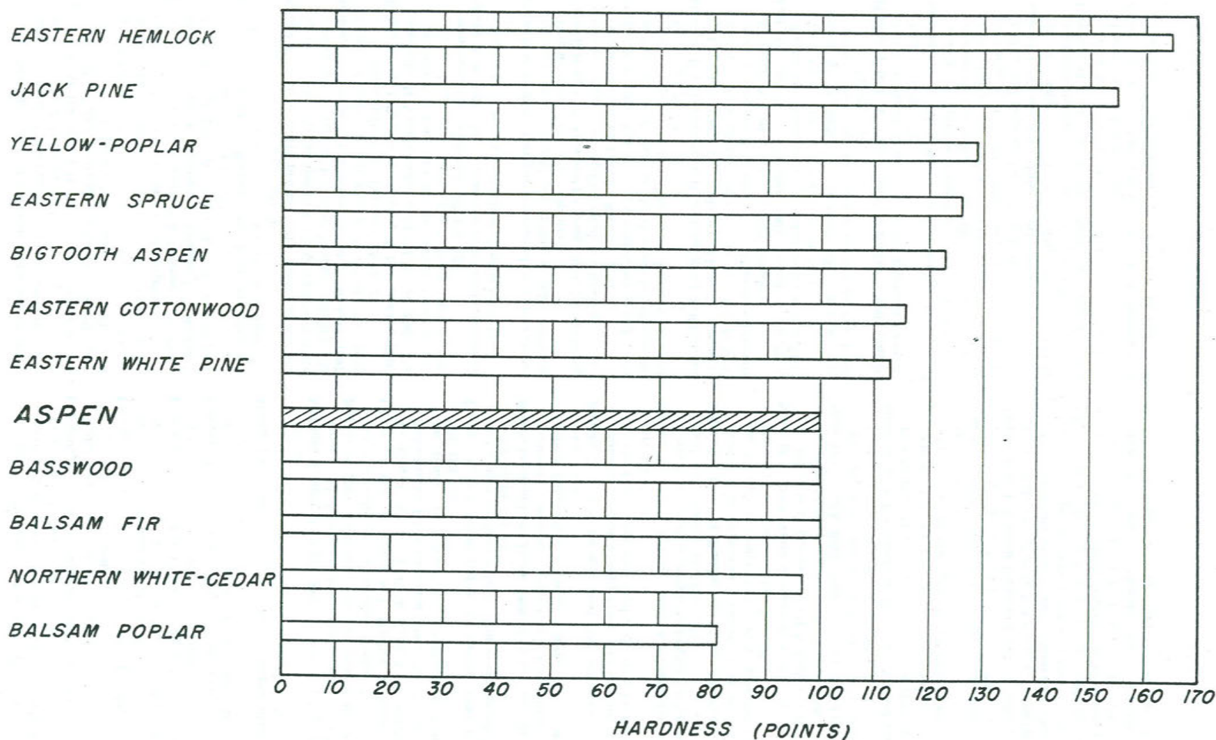
Figure 6.--Average hardness of aspen compared with several other species. Aspen is a soft hardwood. It is suitable for uses where softness rather than hardness is desired.
