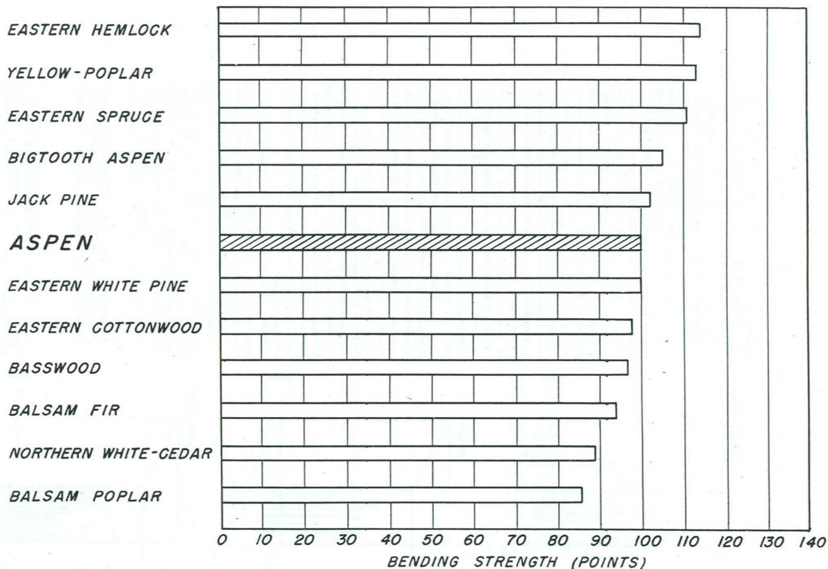
Figure 3.--Average bending strength of the clear wood of aspen compared with several other species.
