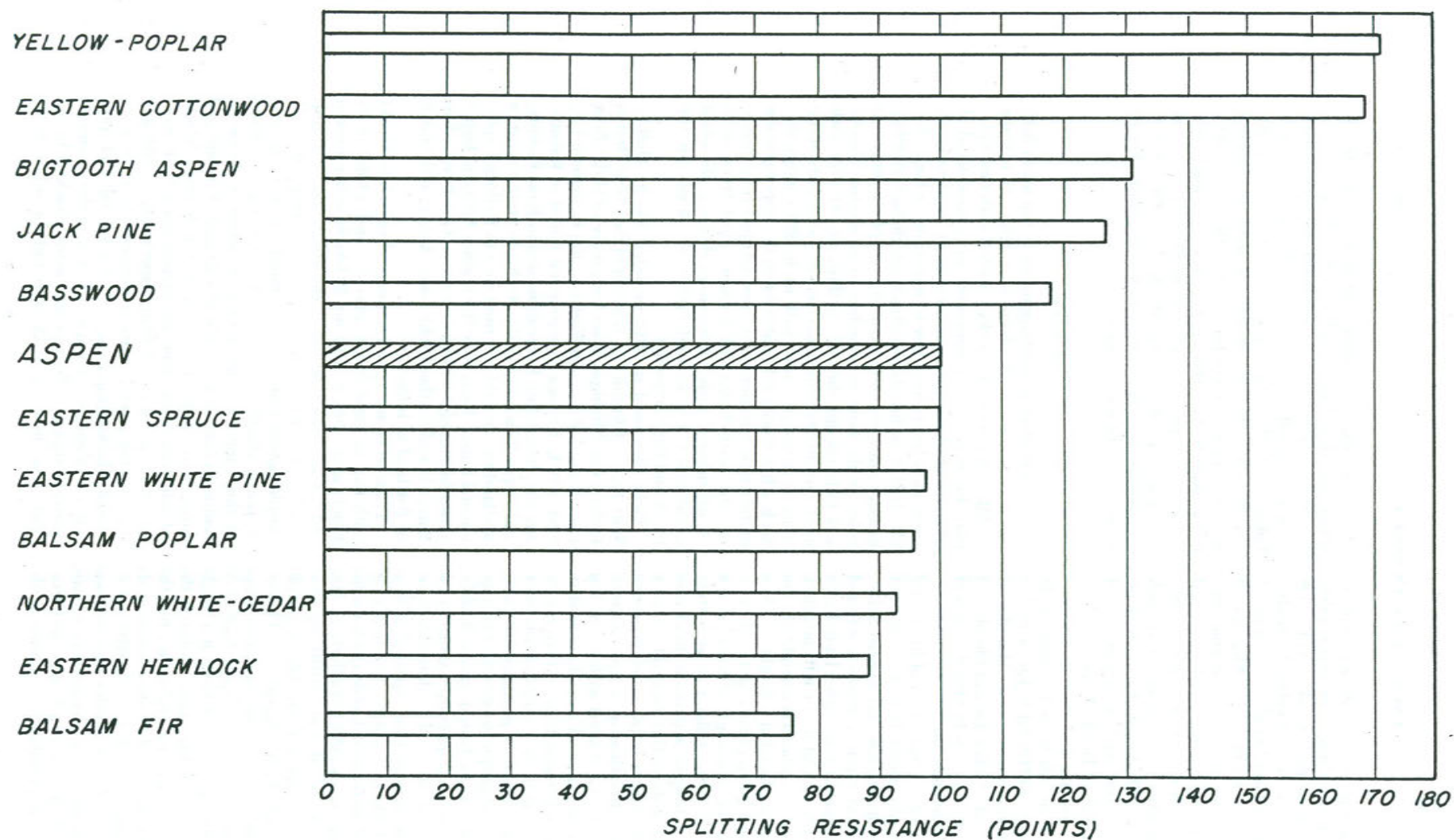
Figure 9.--Comparison of the splitting resistance of the clear wood of aspen with that of several other species.
