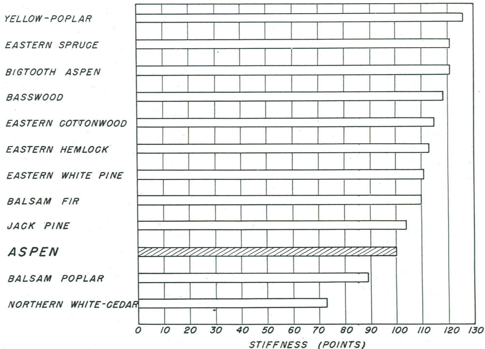
Figure 7.--A comparison of the average stiffness of the clear wood of aspen with several other species.
