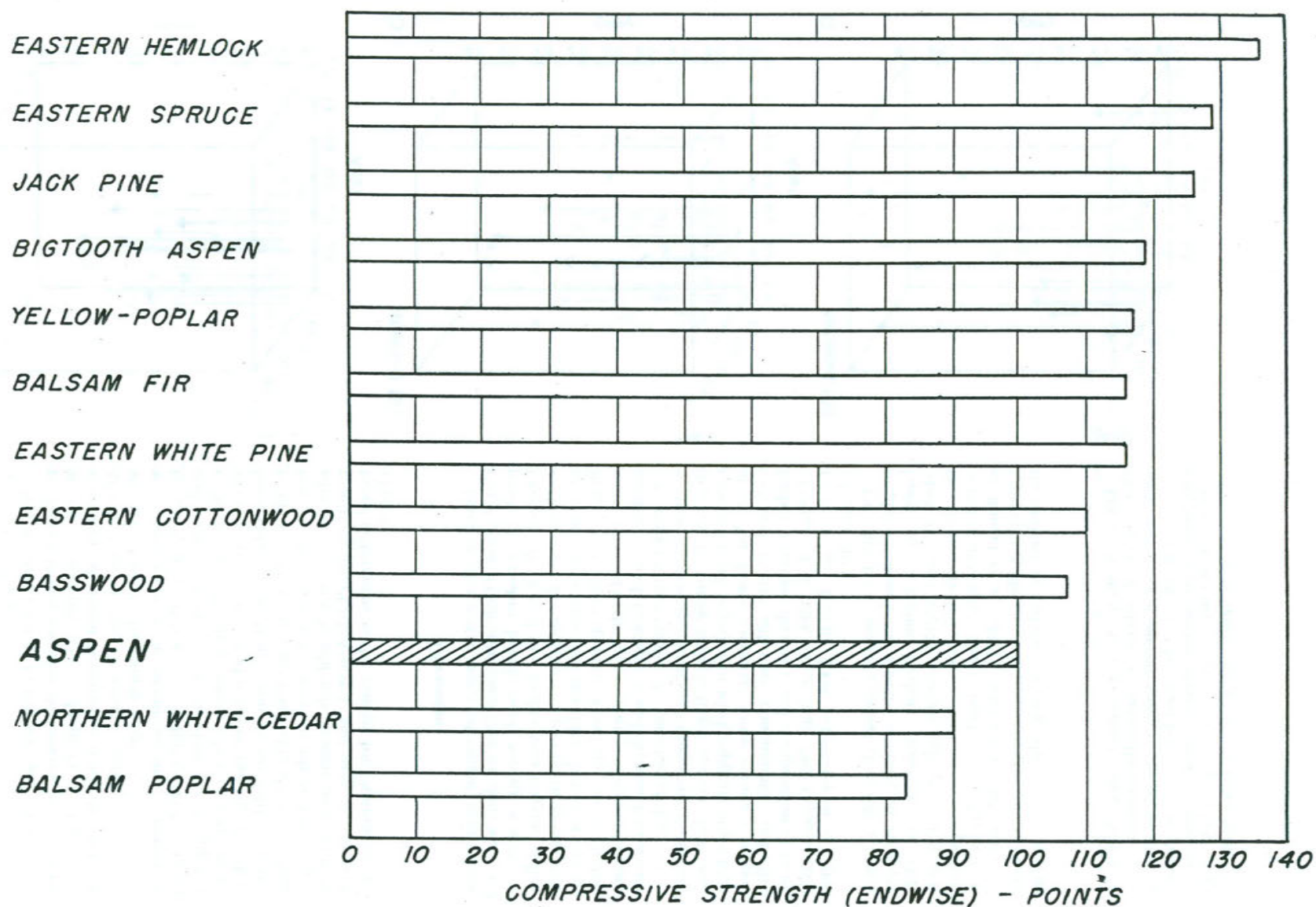
Figure 4.--Average compressive strength (endwise) of the clear wood of aspen compared with several other species.
