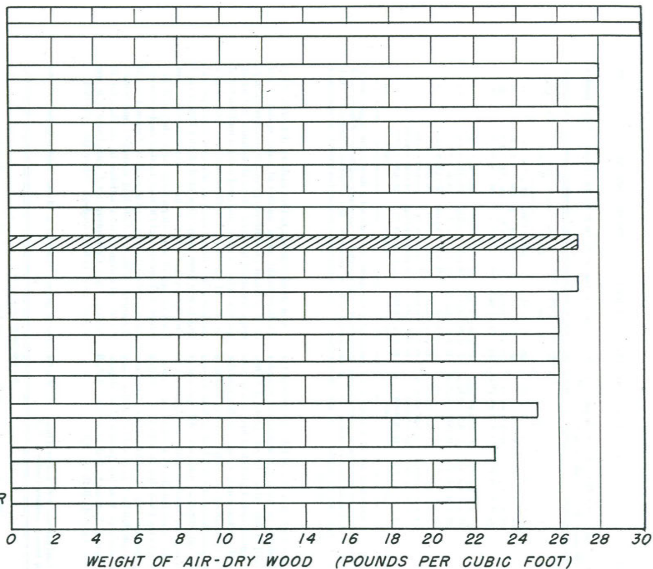
Figure 1.--Weight of air-dry aspen, 12 percent moisture content, compared with the weight of several other species.
