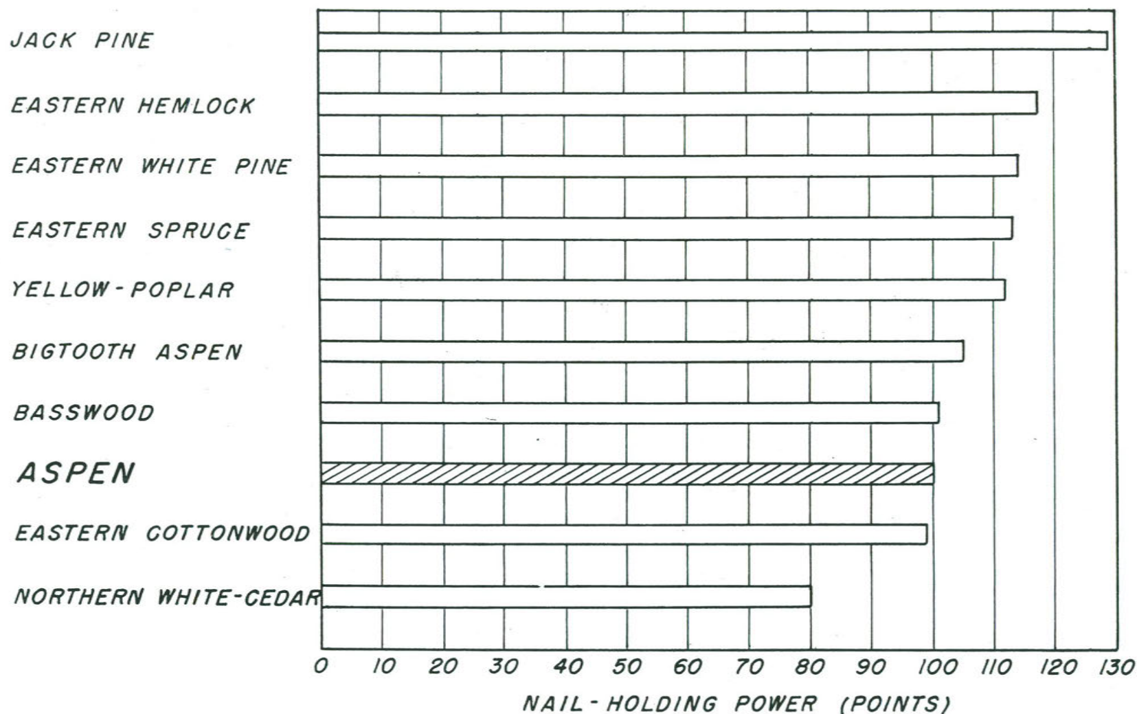
Figure 8.--The nail-holding power of aspen compared with that of several other species.
