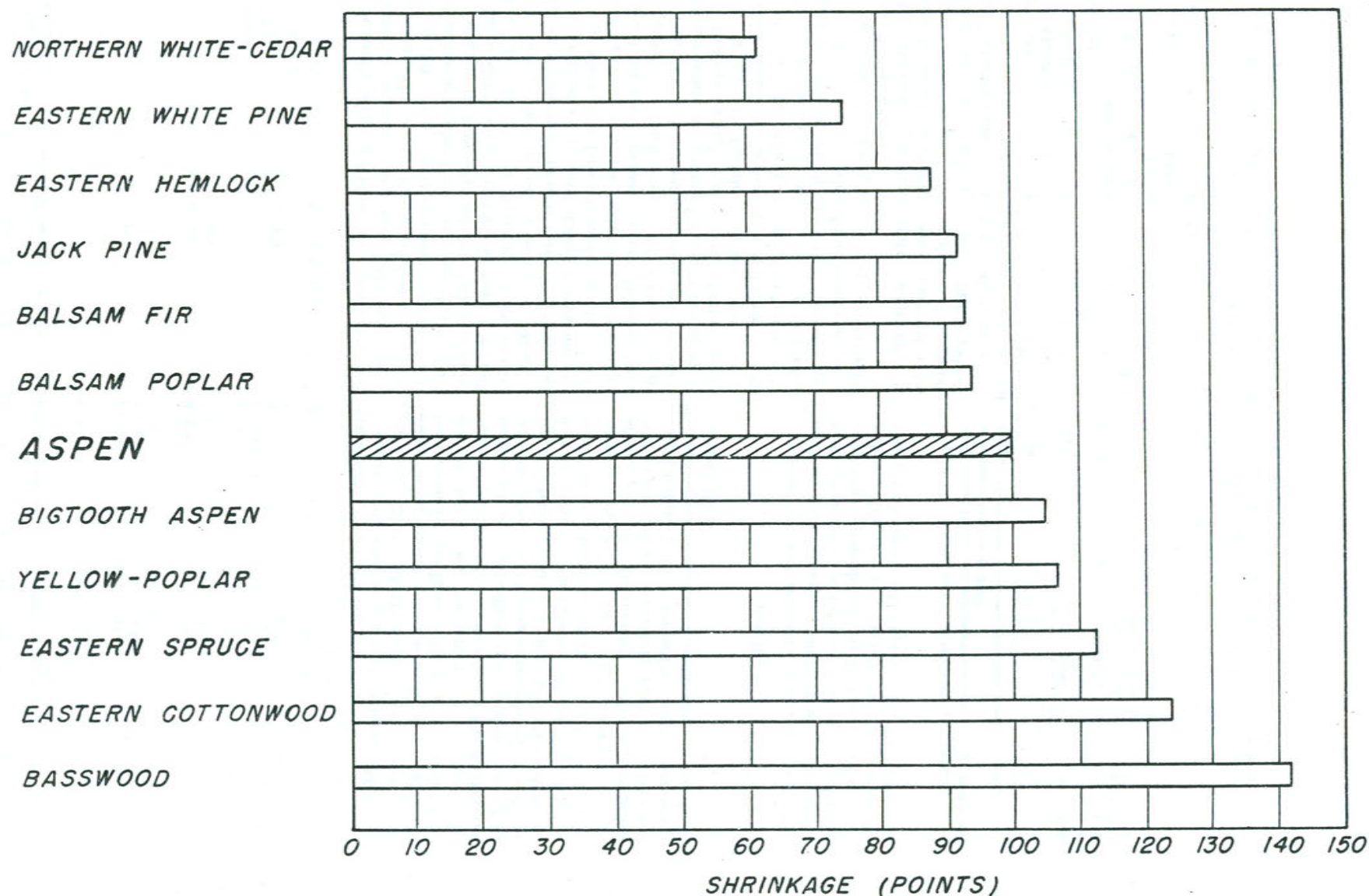
Figure 2.--Comparison of the average shrinkage of aspen with several other species.
