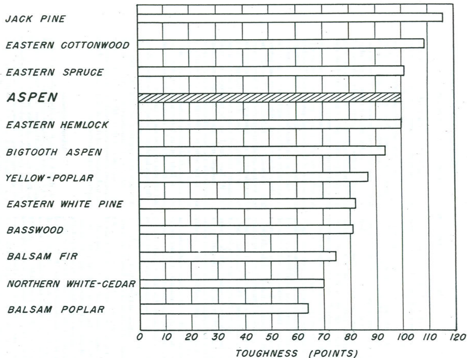
Figure 5.--A comparison of the average shock-resisting ability or toughness of the clear wood of aspen with several other species.
