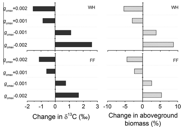
Fig. 9. Results of the sensitivity test. We tested the responses of tree ring \delta^{13}\text{C} and aboveground biomass to g_{c\max 0} . g_{c\max 0} was changed by \pm 0.001 \text{ m s}^{-1} and \pm 0.002 \text{ m s}^{-1} from the finalized values of HF treatments at site WH and FF, respectively. Presented data were the changes from the simulations using original parameter values. The changes of both parameters were significantly correlated ( R^2 > 0.99 and P < 0.01 at both sites; WH: y = 0.032x ; FF: y = -0.002 + 0.035x ; x is the change of \delta^{13}\text{C} (‰) and y is the percent change in aboveground biomass. Therefore, in the tested range, 1‰ error in the tree ring \delta^{13}\text{C} was related to 3.2% and 3.5% of error in aboveground biomass at site WH and FF respectively. We believe it is very easy to detect a 1‰ error in the tree ring \delta^{13}\text{C} , but not easy to detect a 4% error in aboveground biomass.
