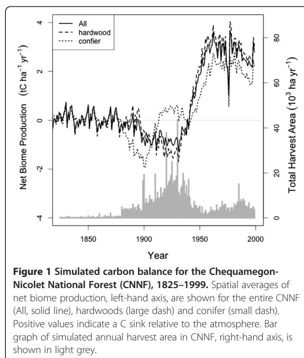
Figure 1 Simulated carbon balance for the Chequamegon-Nicolet National Forest (CNNF), 1825–1999. Spatial averages of net biome production, left-hand axis, are shown for the entire CNNF (All, solid line), hardwoods (large dash) and conifer (small dash). Positive values indicate a C sink relative to the atmosphere. Bar graph of simulated annual harvest area in CNNF, right-hand axis, is shown in light grey.
