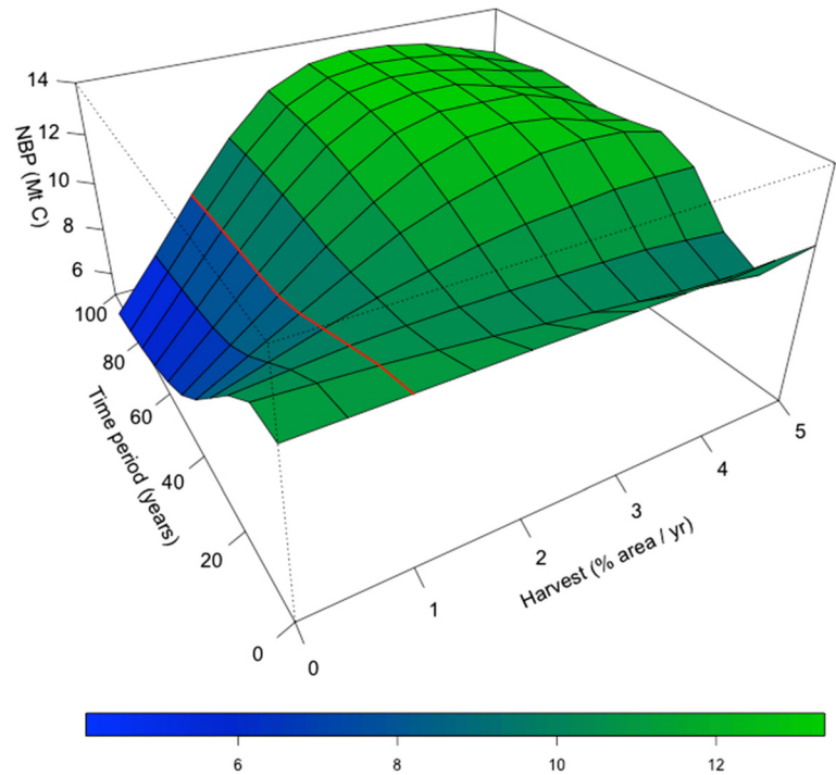
Figure 3 Potential net C uptake for the CNNF in the next 100 years. The x-axis is the percentage of the total area of the CNNF harvested yearly, held constant in every year. The y-axis is the time horizon, or number of 10-year increments. The red line shows NBP when annual harvest is held constant at 1% of the CNNF area.
