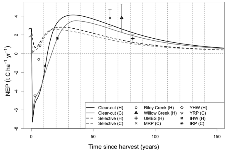
Figure 4 Mean simulated response of net ecosystem production (NEP) to clear-cut (solid lines) and selective (dashed line) harvest over the entire simulation area, for both hardwood (black lines) and conifer (grey line) forest types. Vertical dashed lines denote breakpoints for age-class calculations used in the biological C-budget optimisation. Points show annual estimates of NEP from eight eddy-covariance flux towers in Northern Wisconsin and Michigan in a harvest chronosequence [19], bold symbols denote site means values for sites with measurements in more than two years.
