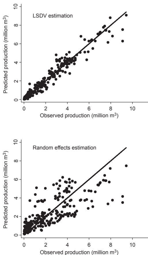
Fig. 3. Observed and predicted production in 25 provinces of China from 1999 to 2009, with the LSDV and random effects estimation. Points on the solid line indicate perfect prediction.
