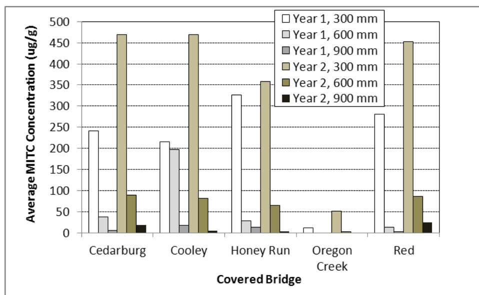
Figure 2. Average MITC concentration in wood samples removed at 300, 600 and 900 mm (12, 24 and 36 in.) from MITC-FUME applications.
