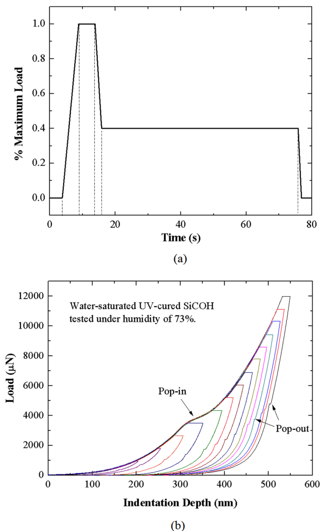
FIG. 3. (a) Load function used in this work, which consists of a 5 s loading, 5 s hold at maximum load, 2 s unload to 40% of the maximum load, 60 s hold at 40% maximum load, 1 s final unload, and a 4 s hold at zero load (The 60 s hold was used to correct the load-depth trace for thermal drift and the 4 s hold was used to assure the load was properly zeroed.); (b) load-depth traces for 20 indents performed on a 500 nm water-saturated UV-cured SiCOH film under humidity of 10%, arrow indicates the occurring of pop-in and pop-out event.
