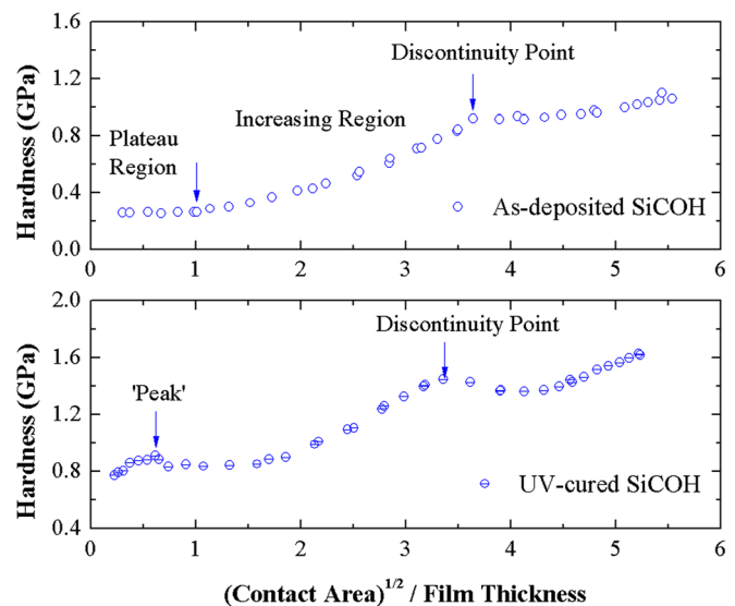
FIG. 6. Measured hardness of SiCOH films as a function of indentation contact radius normalized by film thickness. The data are based on the measurement on 400 °C annealed as-deposited and UV-cured SiCOH under humidity of 10%.
