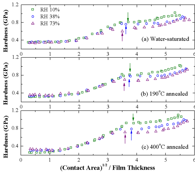
FIG. 7. High loading indentation test measured hardness of different pre-treated as-deposited SiCOH films, as a function of square root of the indentation contact area normalized to the film thickness. Labeled arrows indicate the first occurrence of cracked indent.
