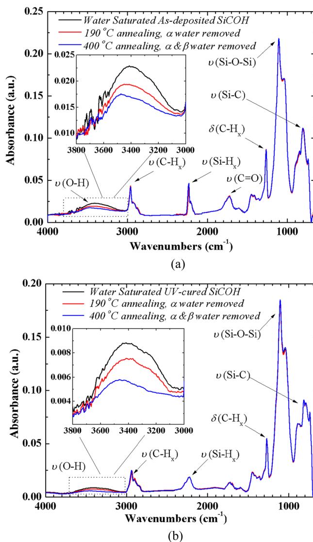
FIG. 2. (a) FTIR spectrum of the water-saturated, 190 °C annealed and 400 °C annealed as-deposited low-k SiCOH film; (b) FTIR spectrum of the water-saturated, 190 °C annealed and 400 °C annealed UV-cured low-k SiCOH film.
