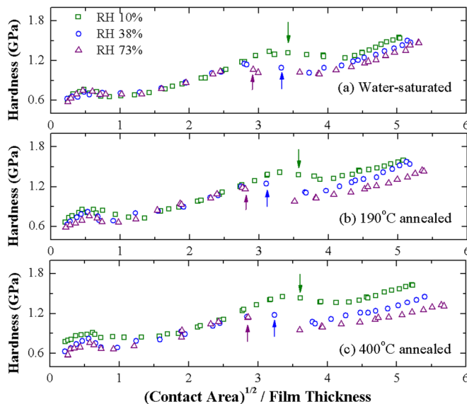
FIG. 8. High loading indentation test measured hardness of different pre-treated UV-cured SiCOH films, as a function of indentation square root of the indentation contact area normalized to the film thickness. Labeled arrows indicate the first occurrence of cracked indent.
