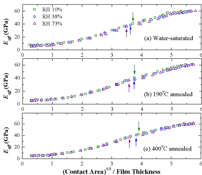
FIG. 10. High loading indentation test measured elastic modulus of different pretreated as-deposited SiCOH films, as a function of square root of the indentation contact area normalized to the film thickness. Labeled arrows indicate the first occurrence of cracked indent.
