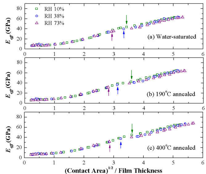
FIG. 11. High loading indentation test measured elastic modulus of different pretreated UV-cured SiCOH films, as a function of square root of the indentation contact area normalized to the film thickness. Labeled arrows indicate the first occurrence of cracked indent.
