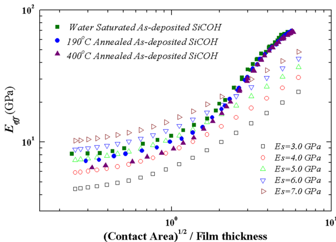
FIG. 5. Comparison of experimental E_{eff} (solid symbols) of the water-saturated as-deposited SiCOH film under a humidity level of 73% with simulated E_{eff} (open symbols) from Stone's model.
