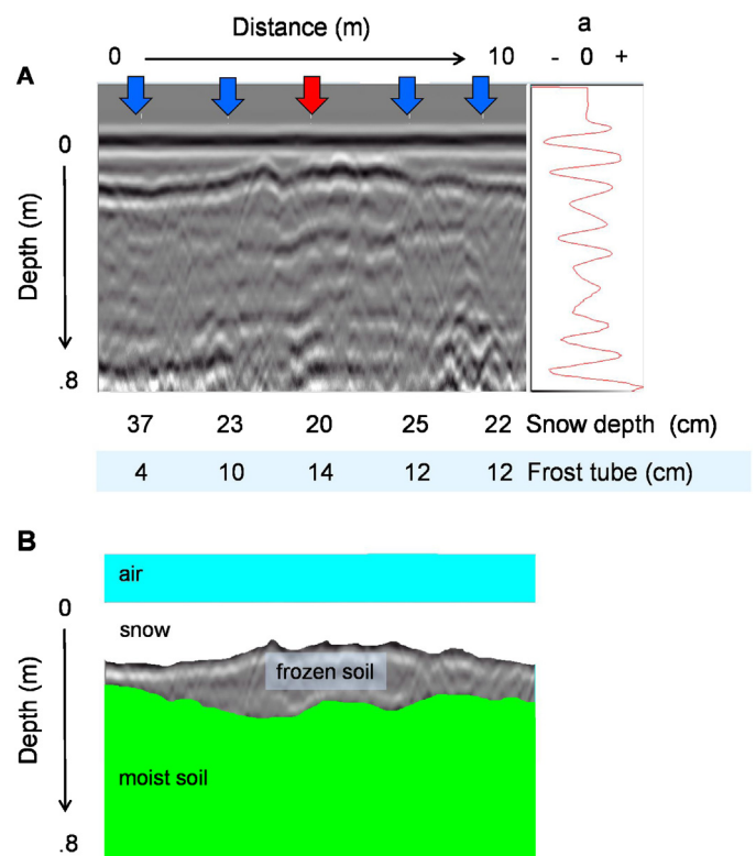
Fig. 6. Radargram collected along a 10 m transect at Sleepers River Watershed, over soils covered with 20–37 cm of snow on January 30, 2012 (A). Arrows indicate the location of frost tubes spaced 2 m apart and the red arrow shows where the waveform diagram on the right was collected. Below each arrow is the snow and frost depth collected at each frost tube. An interpretative schematic summarizing the features observable with GPR is also presented (B).
