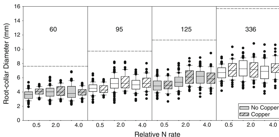
Fig. 2 Box-plots for root-collar diameter data (box represents the 25th and 75th percentiles, horizontal line within the box shows the median, fences are at the 10th and 90th percentiles, and filled circles indicate points outside these percentiles, some of which could potentially be outliers) for each container volume (60, 95, 125, or 336 ml), copper treatment (none = no diagonal fills; copper = diagonal fills), and relative nitrogen (N) rate (0.5, 2, or 4). The horizontal dashed line within each container volume represents the root-collar diameter at which seedlings would reach the 27 % RBI value of South and Mitchell (2006)
