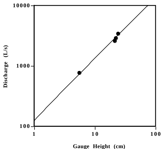
Figure 6 —Plot of discharge as a function of gauge height on a log-log scale. R^2 = 0.990 . Discharge (L/s) = 10^{(2.166 + 0.966 \cdot \text{Log}_{10}(\text{Gauge height cm}))} . Data from Rush Creek (1994) in the Frank Church Wilderness Area, Idaho. Many more data points than those presented here should be obtained before applying this procedure.
