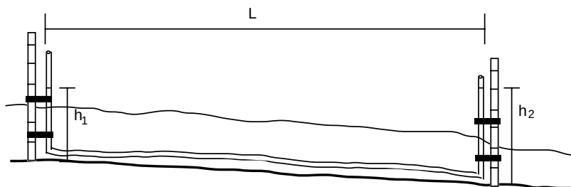
Figure 8 —Diagram showing the calculation of slope by hydrostatic leveling.
