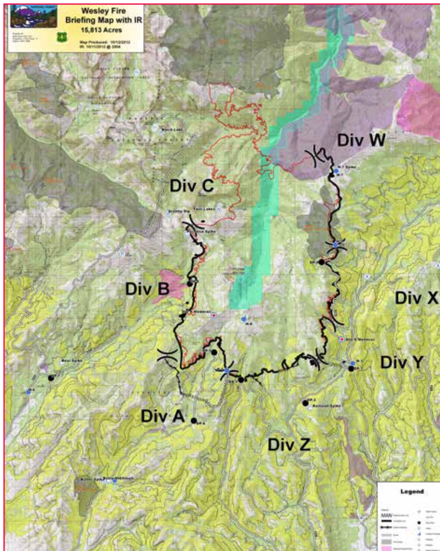
Figure 11. —2012 Wesley Fire, where direct fire suppression was taken on most of the fire except the portion to the north in the Rapid River drainage, which was only monitored because fire spread potential was judged to be low given the time of year (October) and the barriers to fire spread, including prescribed fire treatments.
