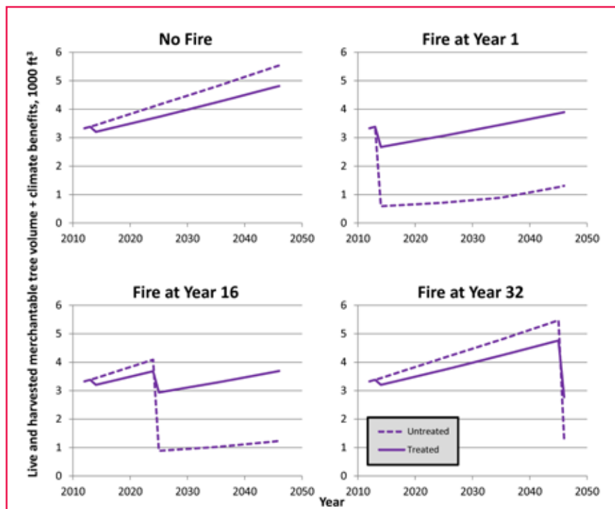
Figure 2. — Trajectories of mean, per acre, merchantable volume (no treatment case), and merchantable volume plus products effects (best treatment case) for 4 fire scenarios, based on 132 plots in Douglas-fir and true fir forests representing 1.2 million acres.
