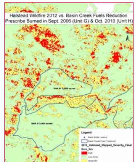
Figure 7. —A portion of the Halstead Fire, where fuels reduction treatment resulted in reduced fire intensity as the larger wildfire burned around these treatment areas.
