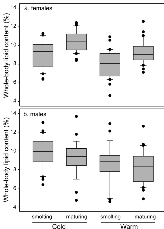
Fig. 8. Whole-body lipid content for smolting and maturing (a) female and (b) male O. mykiss reared under a cold and warm thermal regime. Whiskers represent lines to data that are no more than 1.5 times the interquartile range. Top lines of boxes denote the 75th percentile, bottom lines the 25th percentile, and middle lines the means. Filled circles denote outliers.
