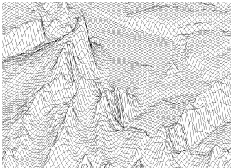
Figure 2. A Digital Elevation Model showing continuous coverage of slope, aspect, and elevation in a raster grid across an entire area. This area is the east side of the Cascade Mountains in west-central Washington State. Each regular grid cell is 1 km on a side. Figure developed and provided by Steve Brown at the University of Montana.
