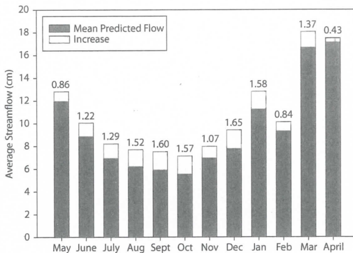
Figure 3.4 Mean monthly changes in water yield during the first 4 postcutting years on Coweeta WS 7. (Modified from Swank et al., 1982)
