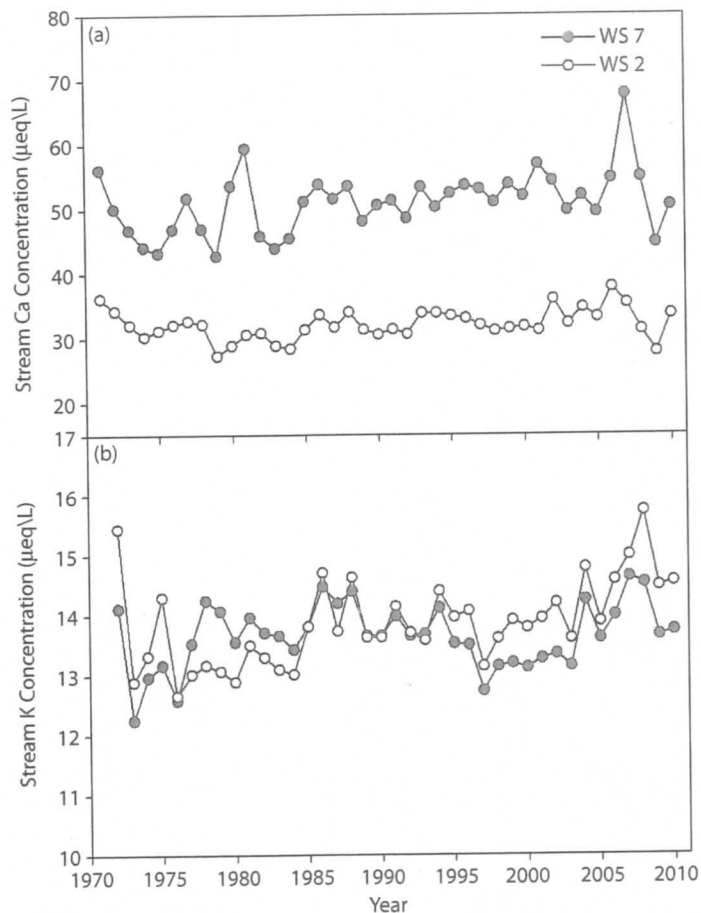
Figure 3.5 Mean annual concentrations of Ca (a) and K (b) in streamwater of WS 7 and WS 2 during calibration (1971–1976), treatment activities (1976–1977), and postharvest period (1978–2010).
