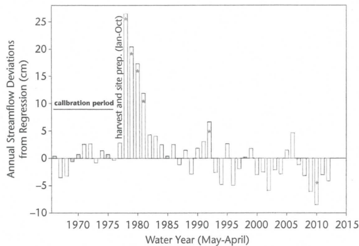
Figure 3.3 Annual deviations in streamflow on WS 7 prior to and following clearcutting and commercial logging at Coweeta Hydrologic Laboratory, 1967–2012. * Denotes significant change; p < 0.05 .
