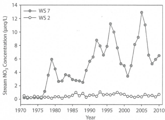
Figure 3.7 Mean annual concentrations of \text{NO}_3 in streamwater of WS 7 and WS 2 during calibration (1971–1978), treatment activities (1976–1977), and postharvest period (1978–2010).
