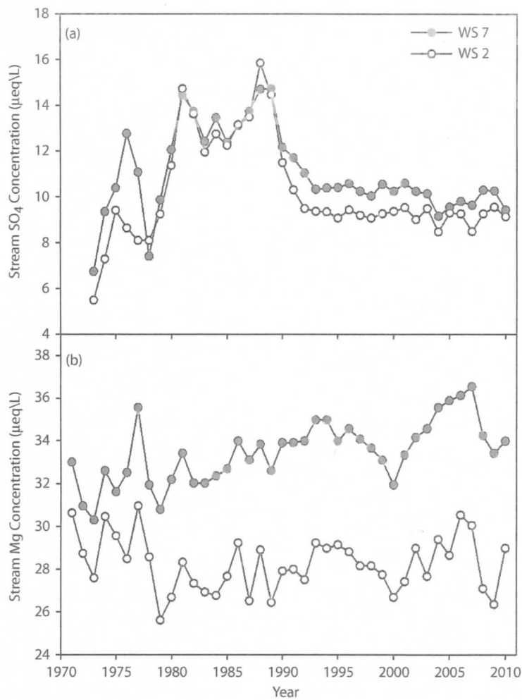
Figure 3.6 Mean annual concentrations of \text{SO}_4 (a) and Mg (b) in streamwater of WS 7 and WS 2 during calibration (1971–1976), treatment activities (1976–1977), and postharvest period (1978–2010).
