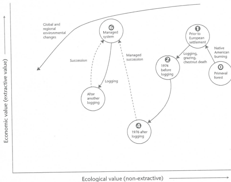
Figure 14.2 Hypothetical trajectories of change in ecological and extractive values of WS 7 with adaptive management of post-logging succession. Solid lines are human-caused changes and dashed lines are successional changes with management based on ecosystem research and predictions of environmental change.
