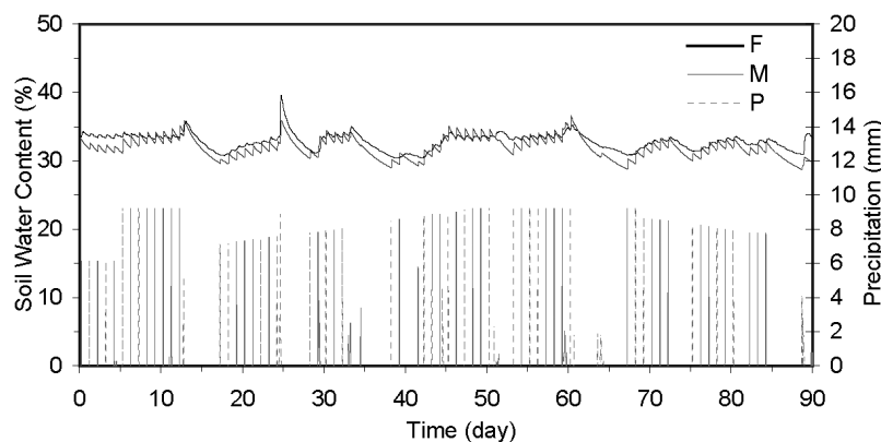
Figure 3. Soil moisture measured from the site (F) and from the model simulation (M). Precipitation (P) here included both rainfall and landscape irrigation
