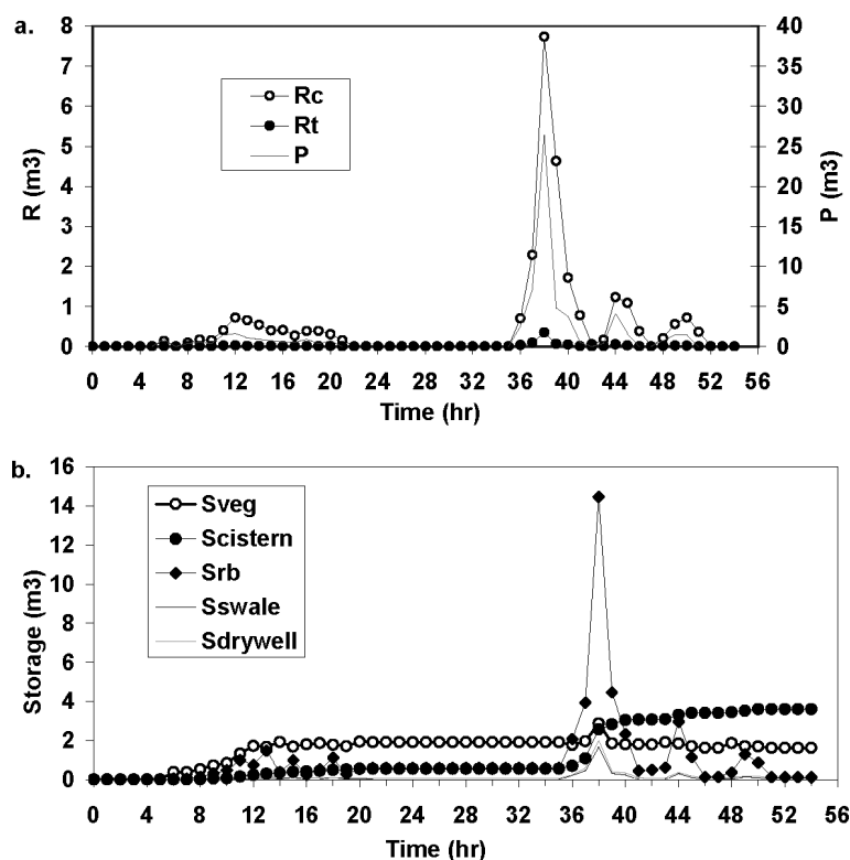
Figure 7. Runoff processes for a 50-year storm event. The storm started midnight on 1 February 1998. This storm lasted 45 h with two separate events and brought a total of 65.3 mm rainfall. (a) Precipitation P and runoff to the street for both treatment R_t and control R_c sites. (b) Surface retention storage dynamic change on the treatment site. Here S means storage. The S 's subscript denotes the BMP's name
