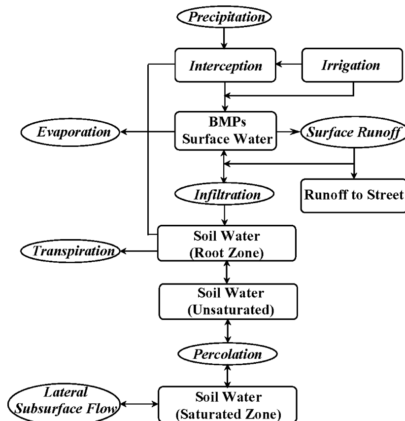
Figure 2. Model flow chart of hydrologic processes at the residential scale
